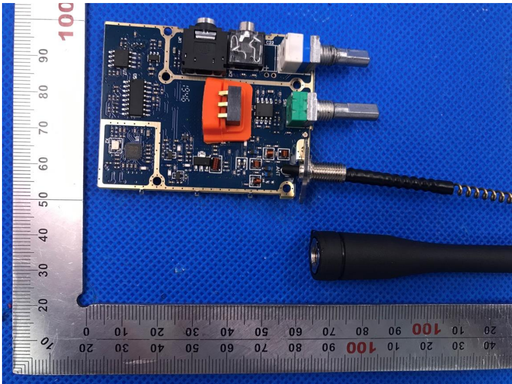
ANTENNA CLOSEUP-2
