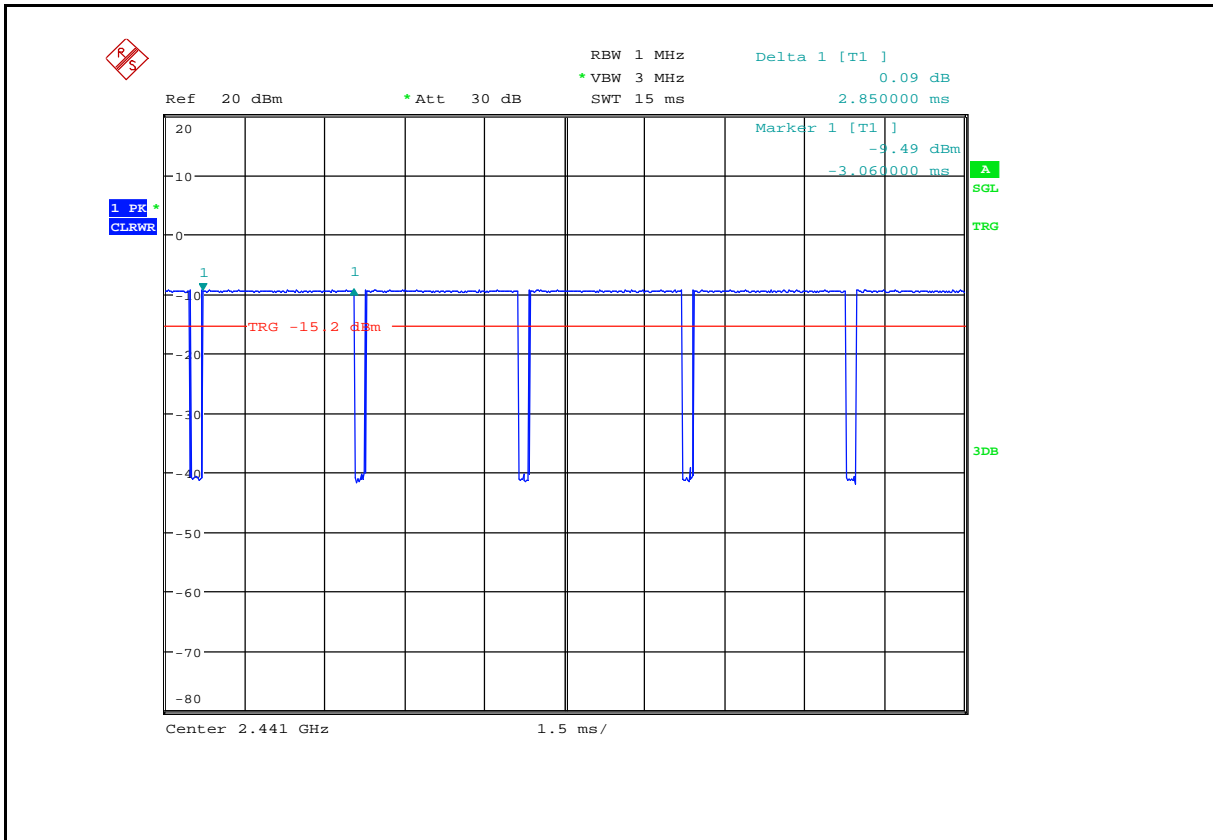
Dwell Time_3DH1_2441
