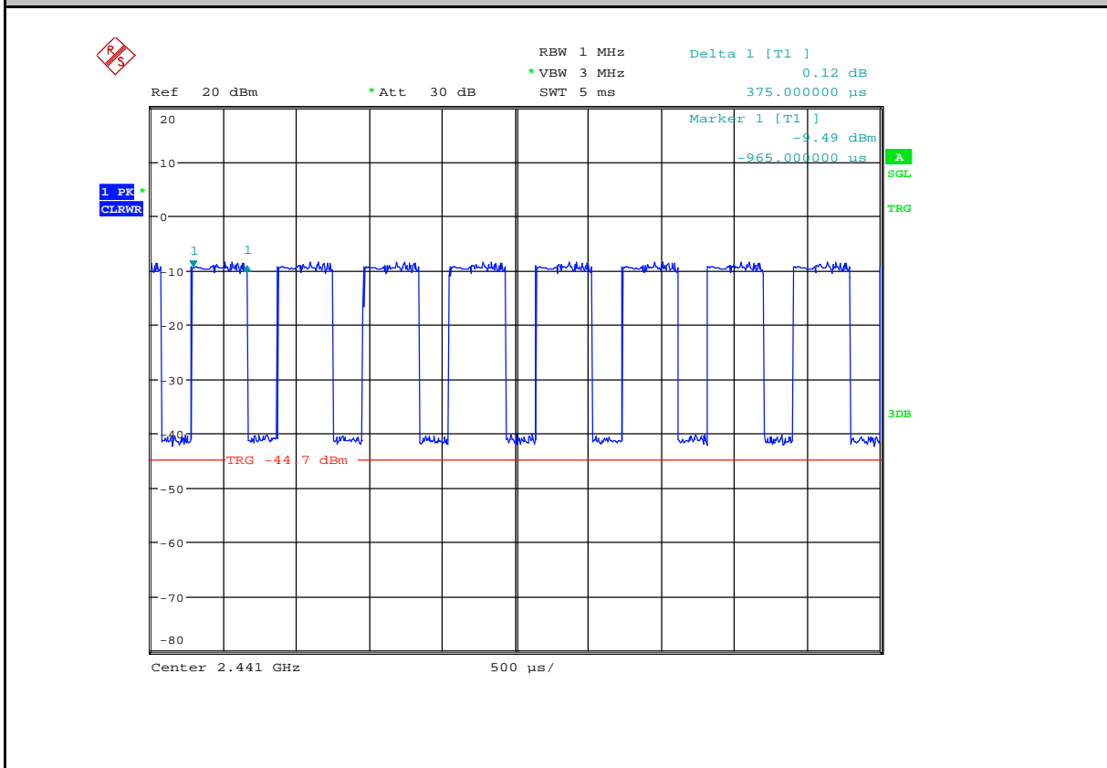
Dwell Time_3DH3_2441
