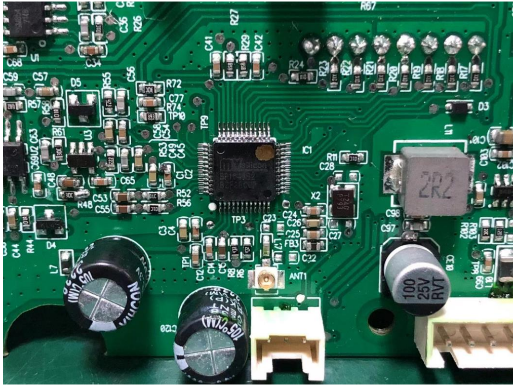
Internal Photos M/N: PATHFINDER™ GO
