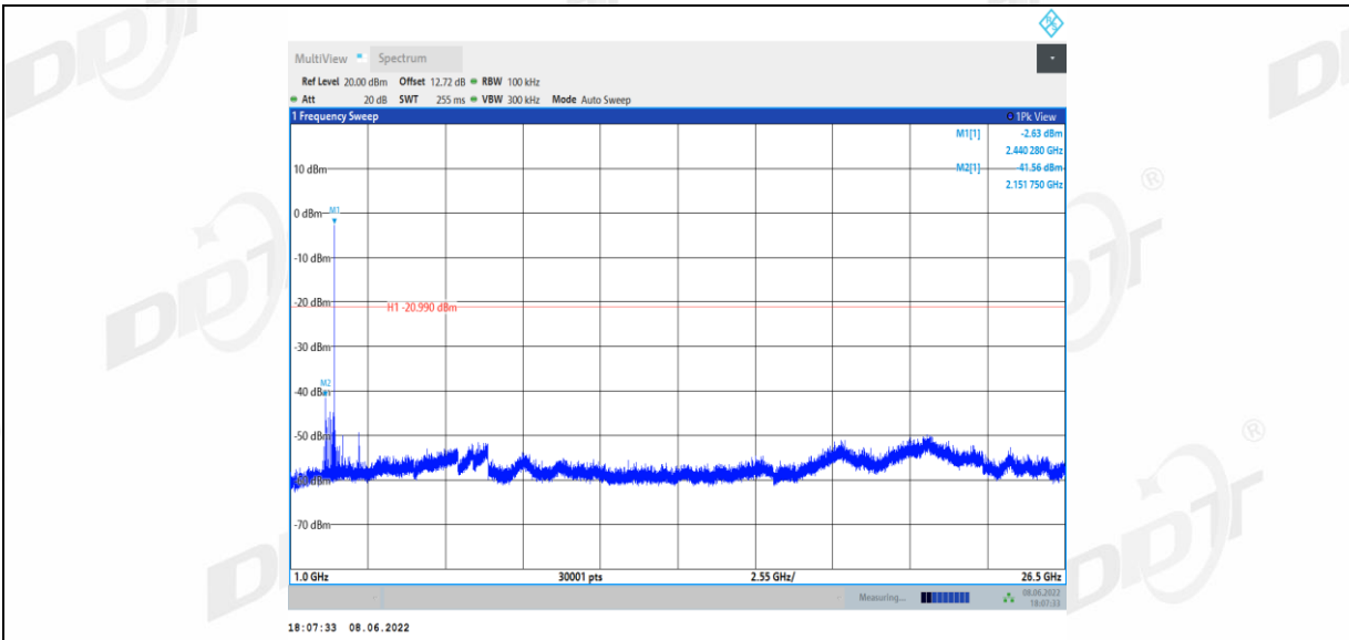
BLE_1M_Ant1_2480_0~Reference
