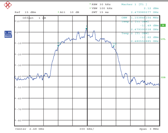
8-DPSK Mode 2480MHz
