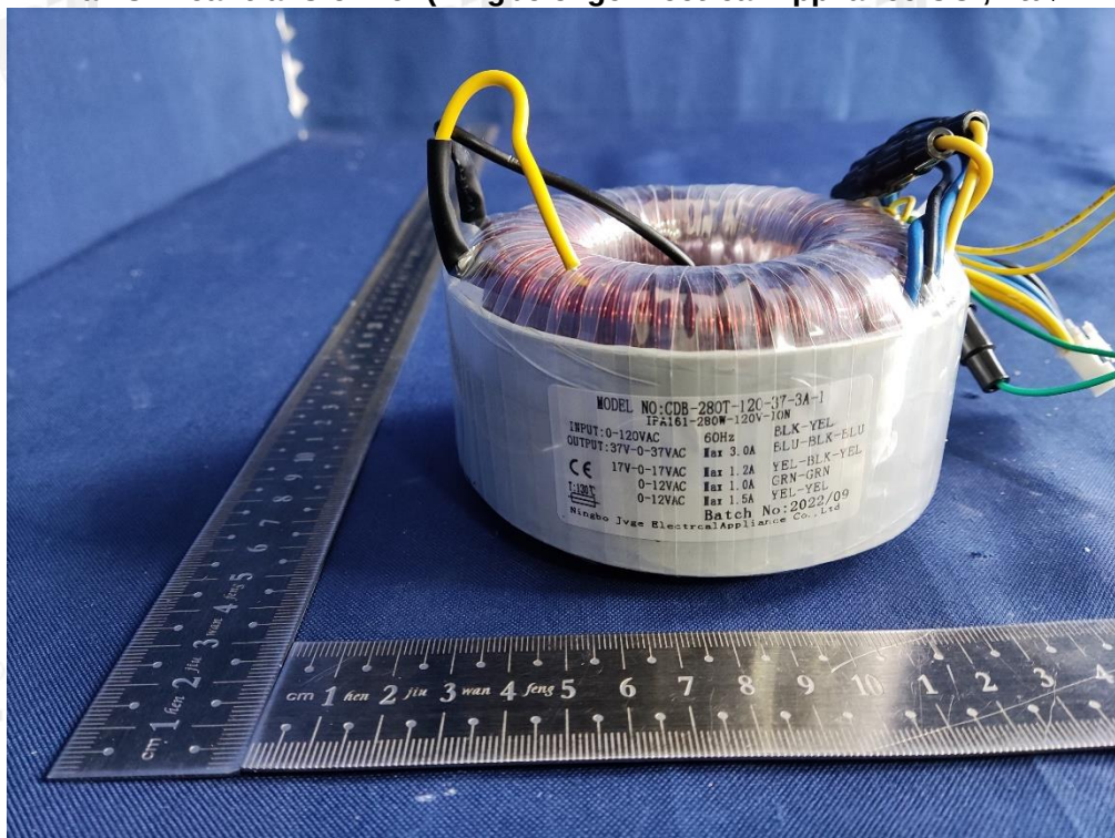
Mains linear transformer (Ningbo Jvge Electrical Appliance CO., Ltd)
