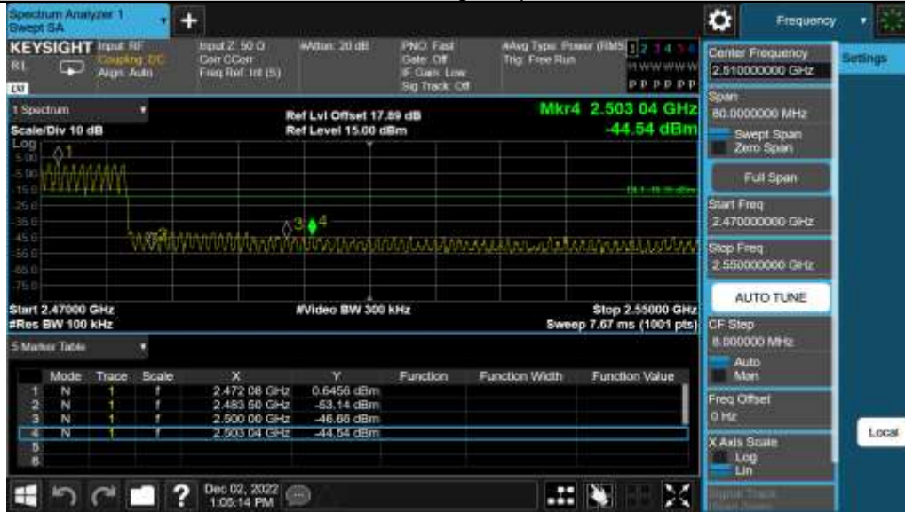
DH5_Ant1_High_Hop_2480
