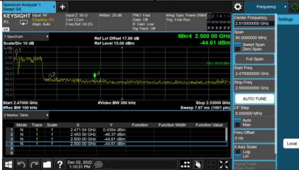
2DH5_Ant1_High_Hop_2480
