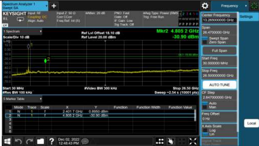
2DH5_Ant1_2402_30~26500
