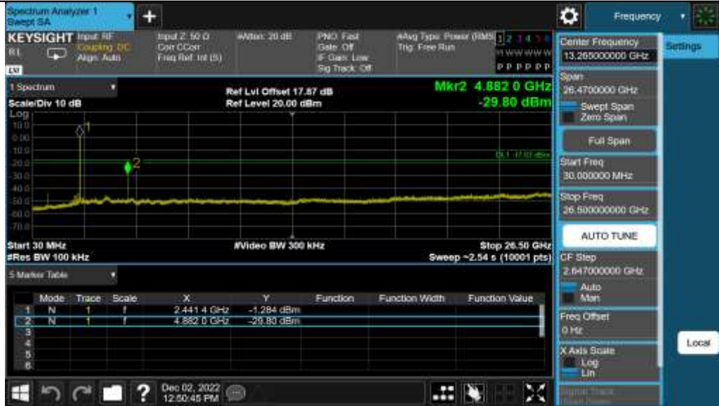
2DH5_Ant1_2441_30~26500
