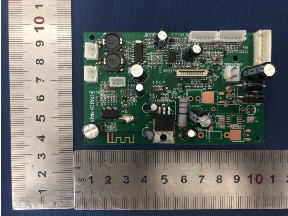
(PROJECTOR PA, iPA119AC charging circuit difference)
