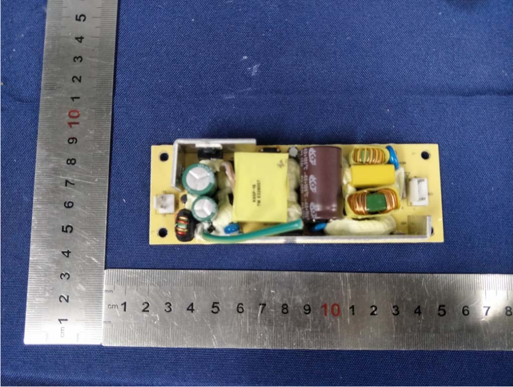
(Power board: Guanjin / K65P160410-X3)
