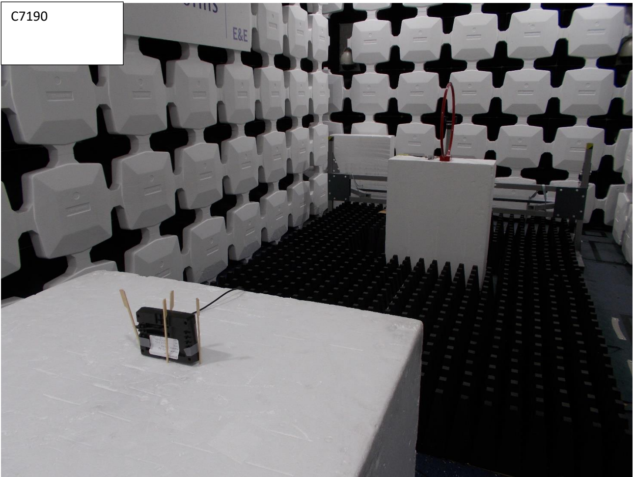
Magnetic field emissions 9kHz to 30MHz – perpendicular orientation
