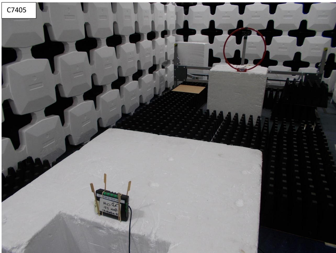
Magnetic field emission 9kHz to 30MHz
