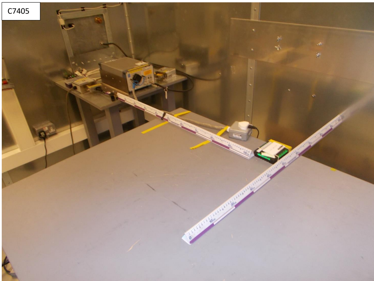
AC Mains Conducted Emissions
