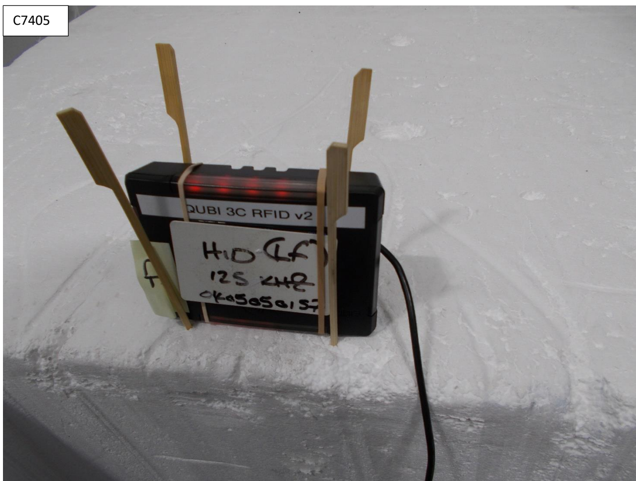
EUT Setup – Radiated emissions
