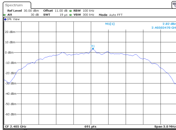
Zigbee_Ant1_2405_0~Reference
