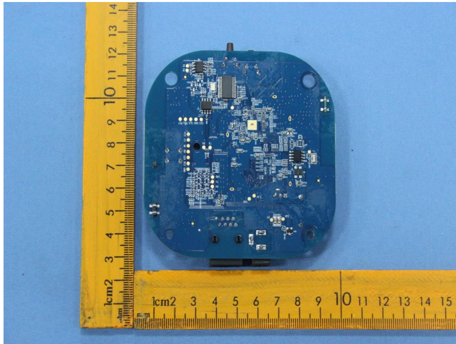
Optional PCB, without power key S3
