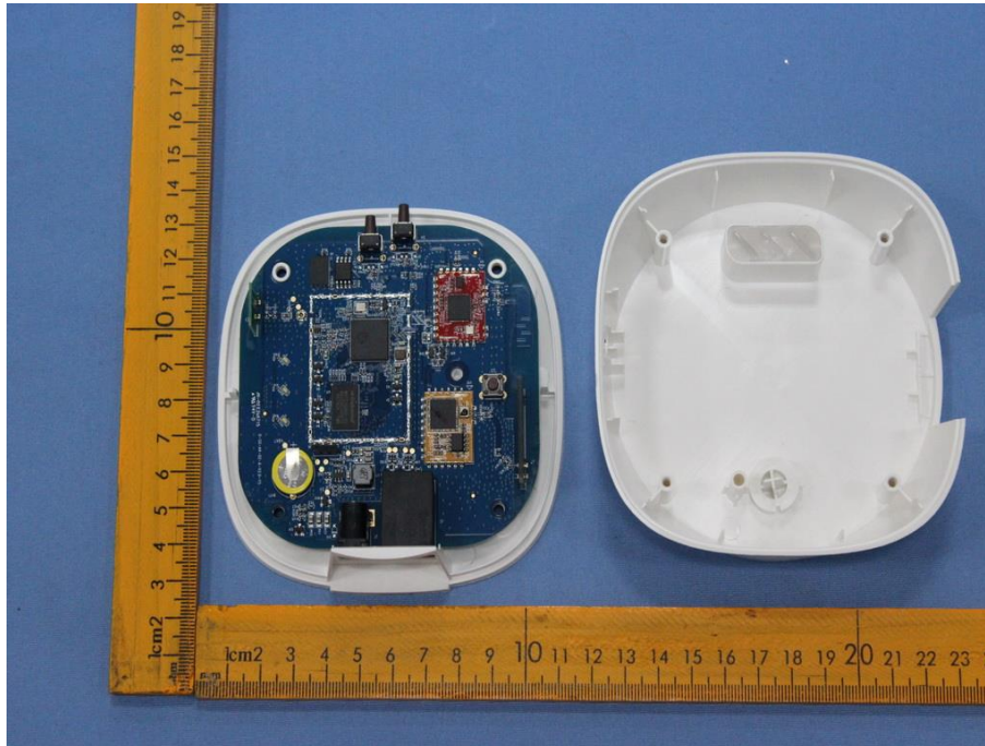
Optional PCB, with power key S3
