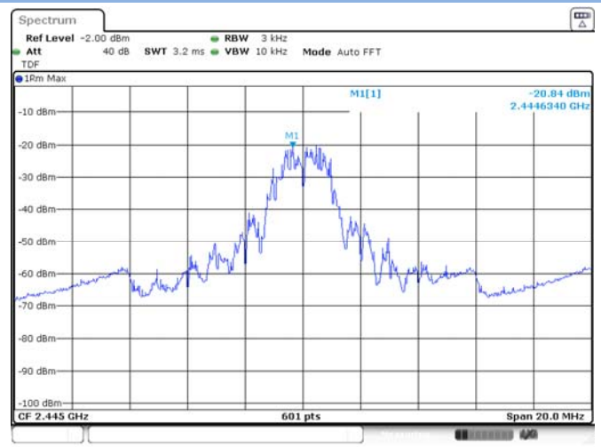
O-QPSK MIDDLE CHANNEL
