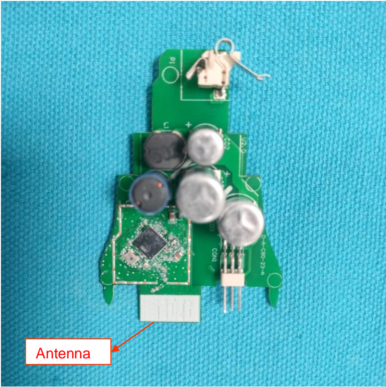
Internal View of EUT-6
