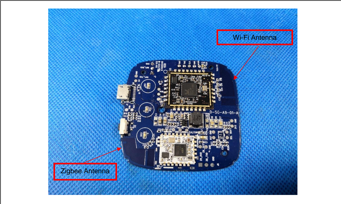
Details of: PCB component side view for model 7B-GW-ZWA-H0-01
