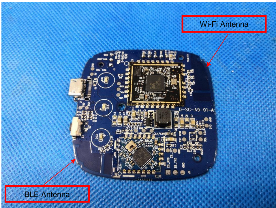
Details of: PCB component side view for model 7B-GW-BWA-H0-01
