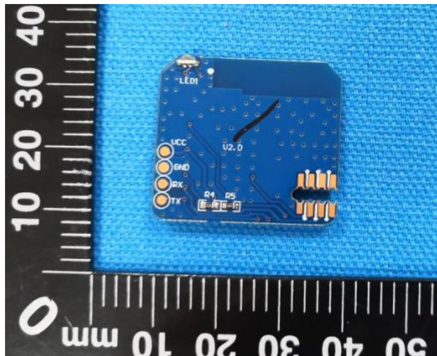
Detail View of WIFI module-2
