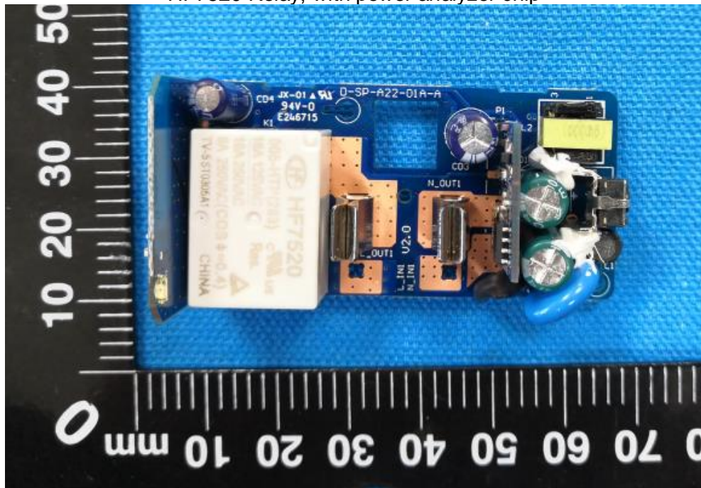
HF7520 Relay, with power analyzer chip
