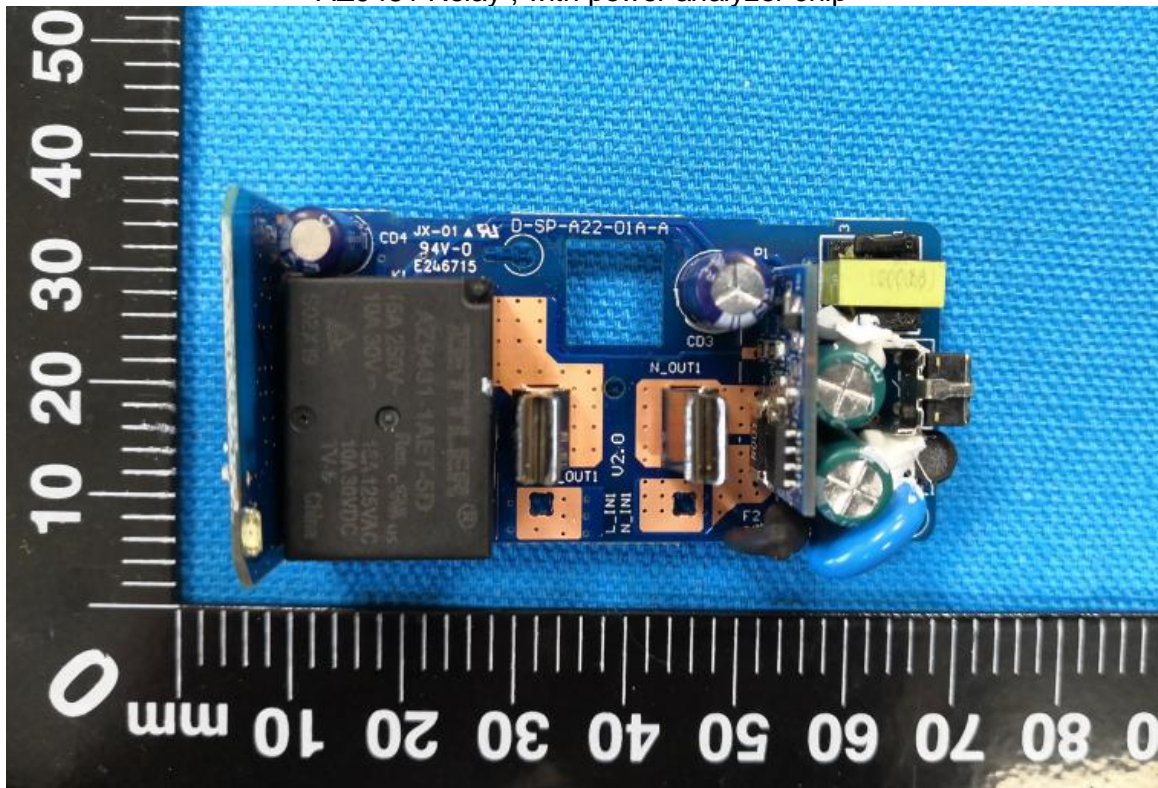
AZ9481 Relay , with power analyzer chip
