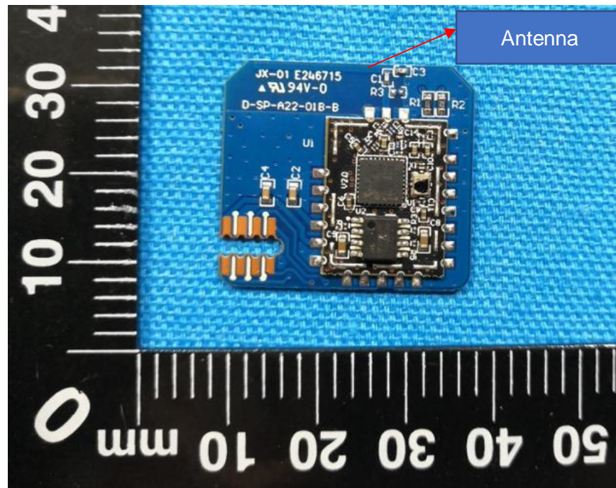
Detail View of WIFI module-2
