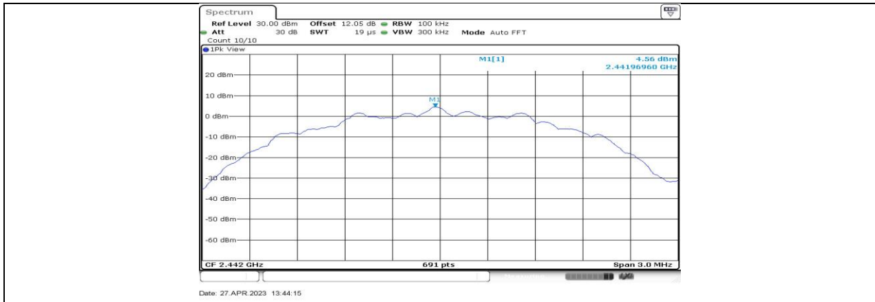
BLE_2M_Ant1_2442_0~Reference
