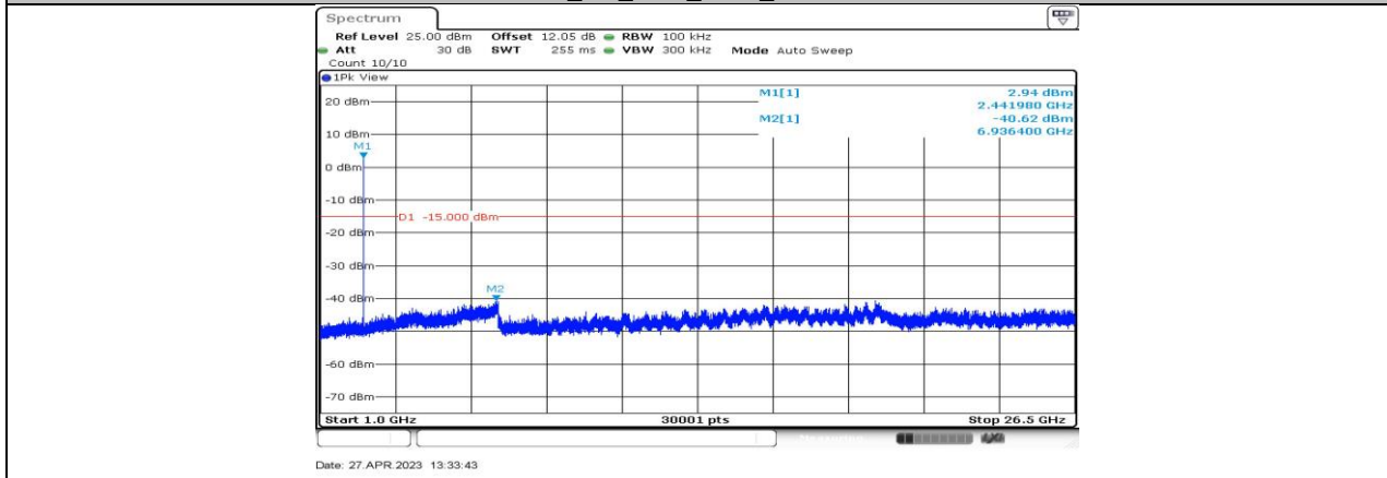
BLE_1M_Ant1_2442_1000~26500
