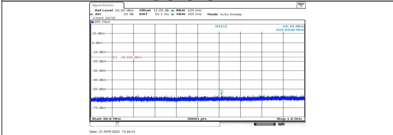
BLE_2M_Ant1_2442_30~1000
