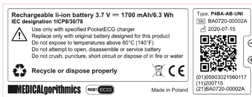
Fig. 6 Label for PocketECG battery (type P4BA-AB-UNI)
