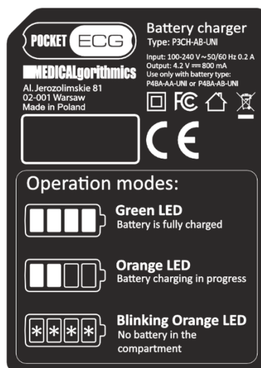
Fig. 4 Label for PocketECG battery charger (type P3CH-AB-UNI) - bottom view
