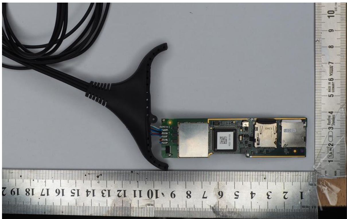
Fig. 6 P4TR-CA-ADS HDI2 (top view )
