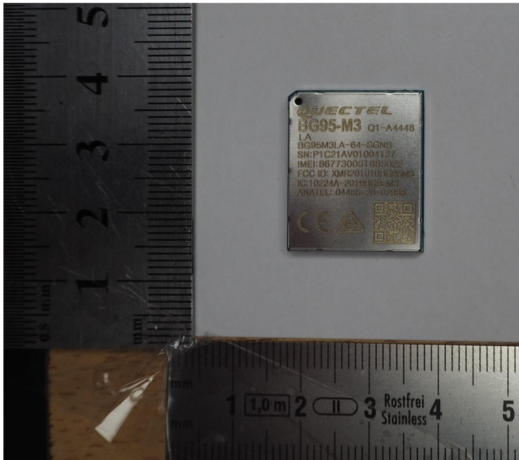
Fig. 7 BG95-M3 module (top view)
