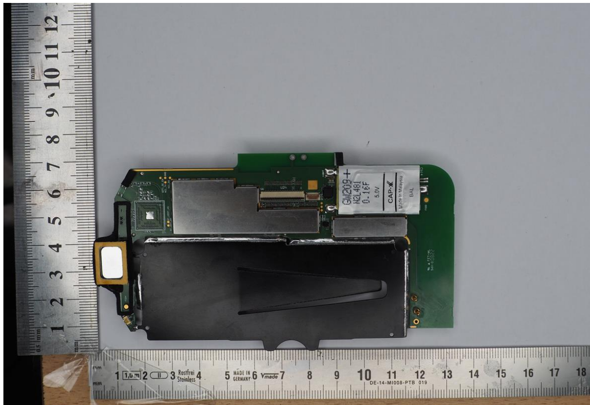
Fig. 3 P4TR-CA-ADS HDI1 (top view)
