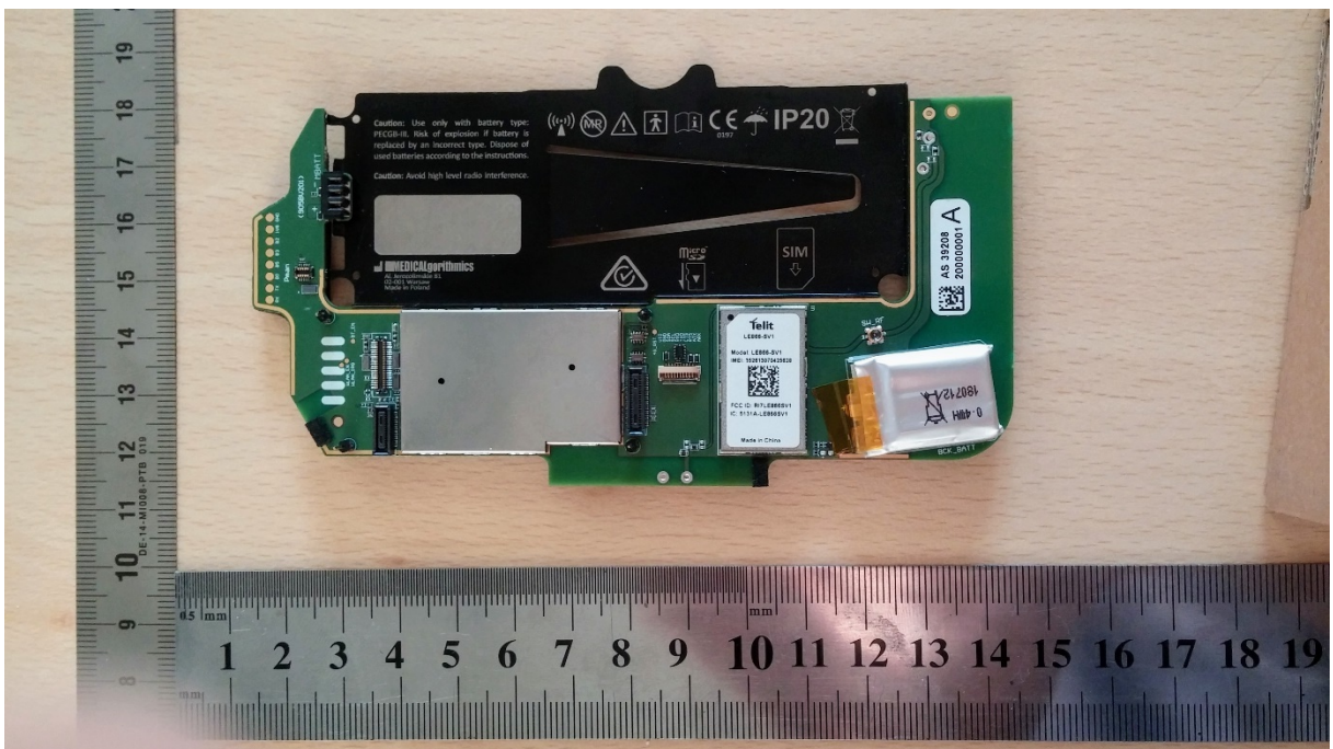
Fig.4 P4TR-AA-ADS HDI1 (bottom view )
