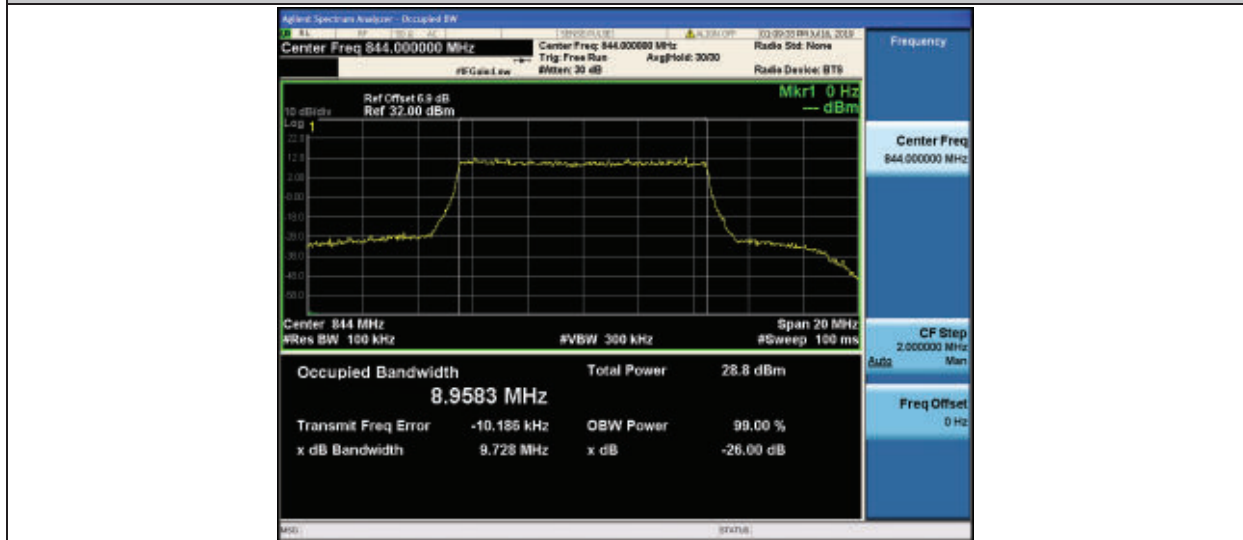
Band26-10MHz-16QAM-26990-50RB#0
