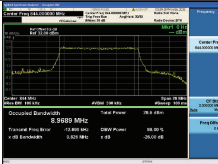
Band26-10MHz-QPSK-26990-50RB#0
