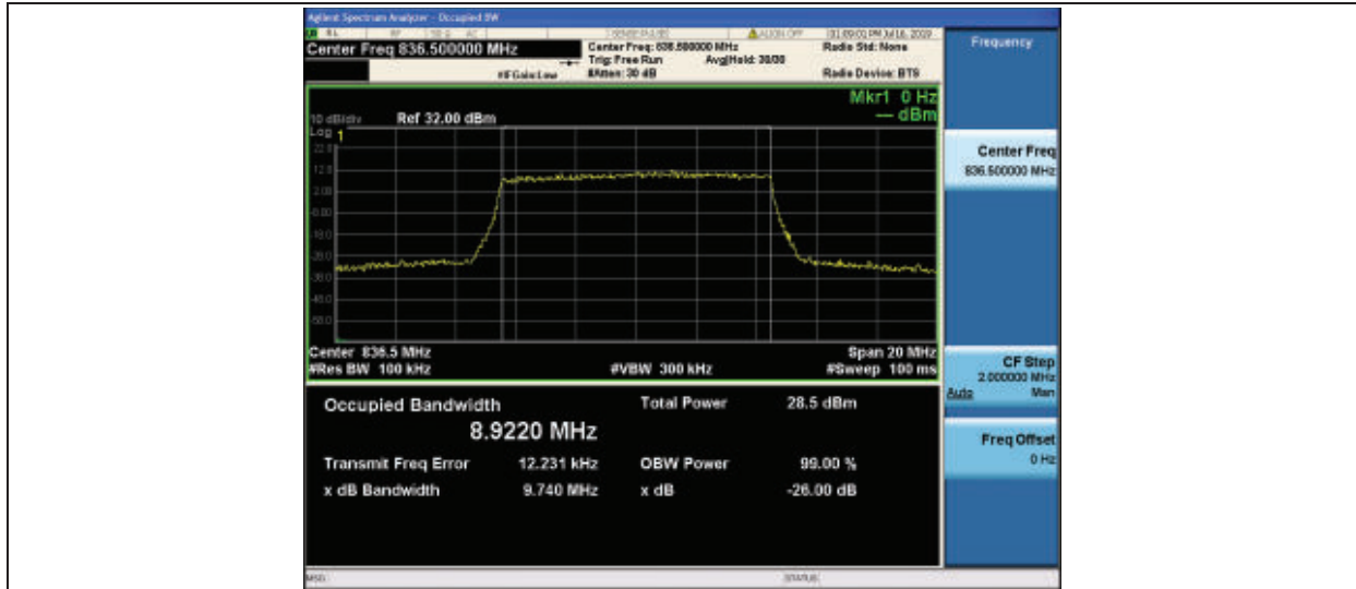
Band26-10MHz-16QAM-26915-50RB#0
