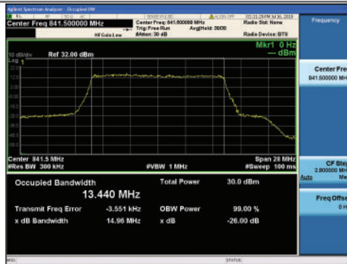
Band26-15MHz-QPSK-26965-75RB#0
