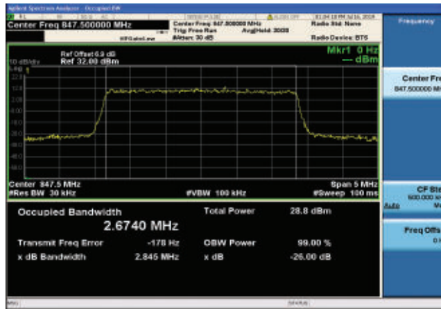
Band26-3MHz-QPSK-27025-15RB#0
