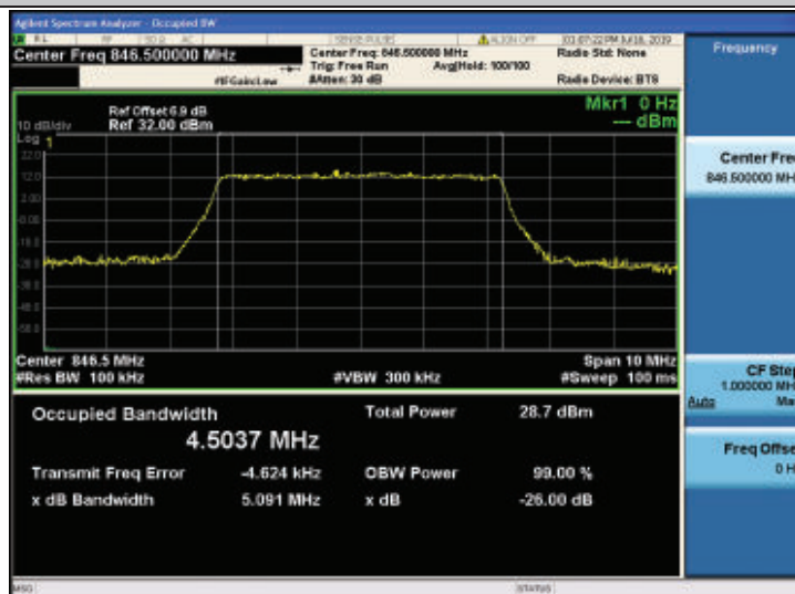
Band26-5MHz-16QAM-27015-25RB#0
