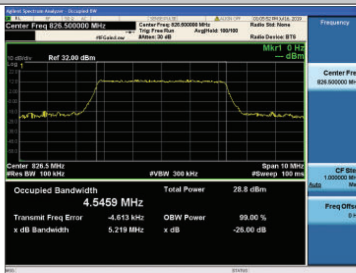
Band26-5MHz-16QAM-26815-25RB#0
