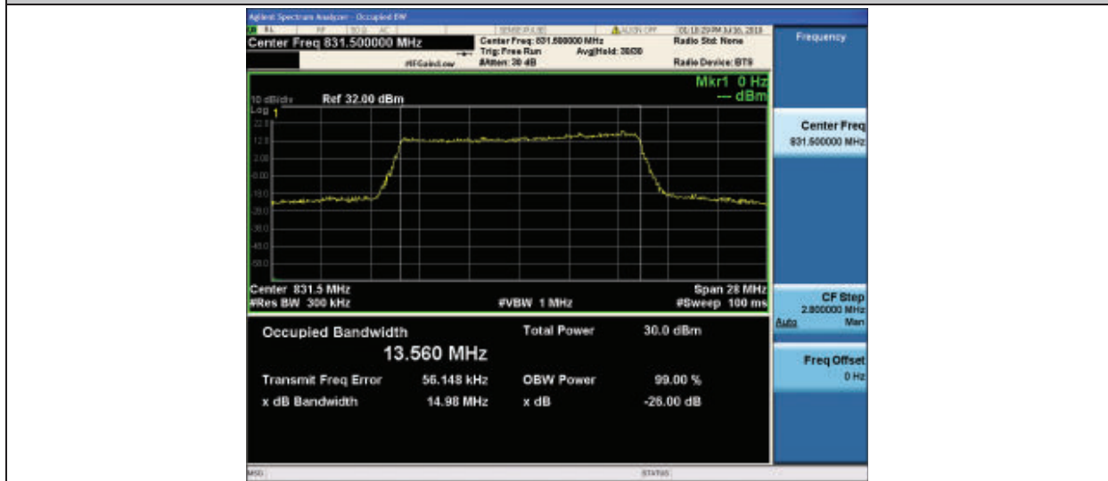
Band26-15MHz-QPSK-26865-75RB#0
