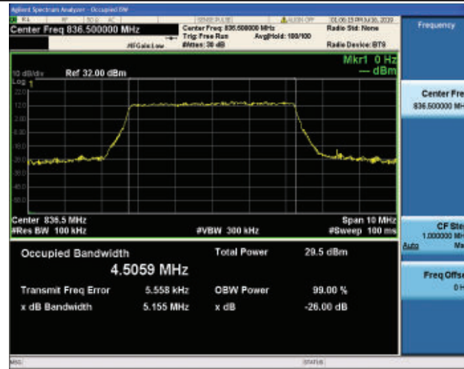
Band26-5MHz-QPSK-26915-25RB#0
