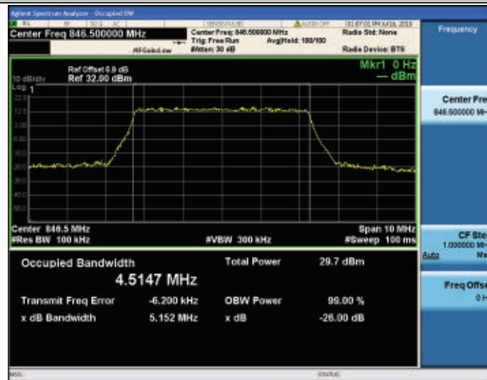
Band26-5MHz-QPSK-27015-25RB#0
