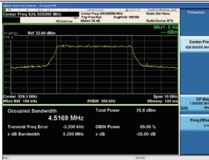
Band26-5MHz-QPSK-26815-25RB#0
