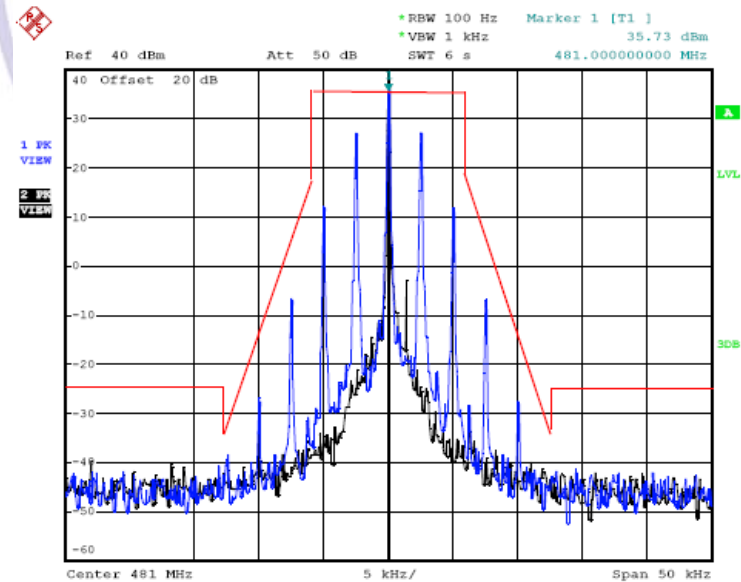
12.5 kHz Channel Spacing, 481.0000 MHz, 2500 Hz Audio Modulation Only
