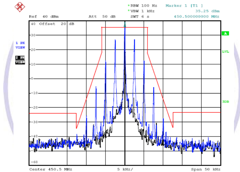
12.5 kHz Channel Spacing, 450.5000 MHz, 2500 Hz Audio Modulation Only
