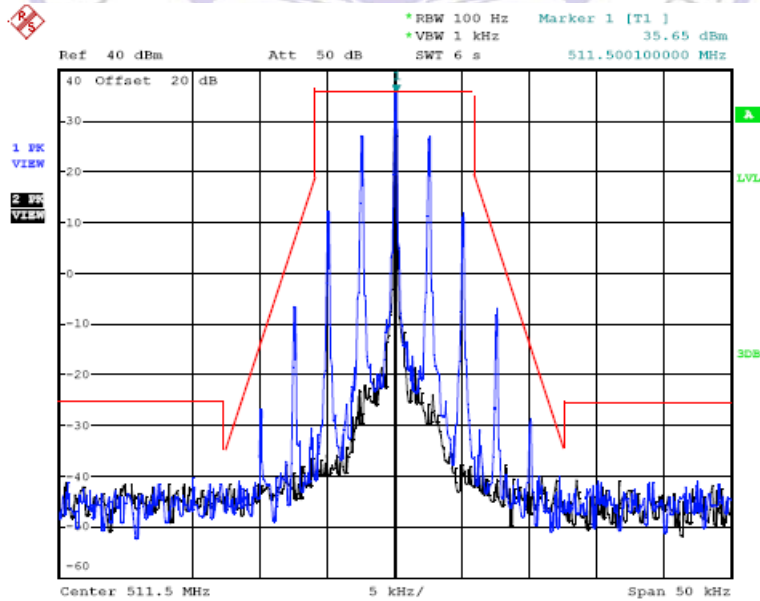
12.5 kHz Channel Spacing, 511.5000 MHz, 2500 Hz Audio Modulation Only
