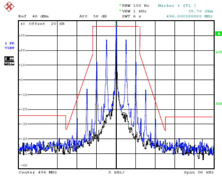
12.5 kHz Channel Spacing, 496.0000 MHz, 2500 Hz Audio Modulation Only
