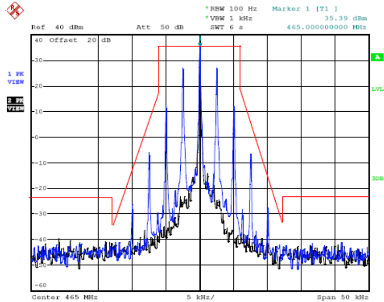
12.5 kHz Channel Spacing, 465.0000 MHz, 2500 Hz Audio Modulation Only
