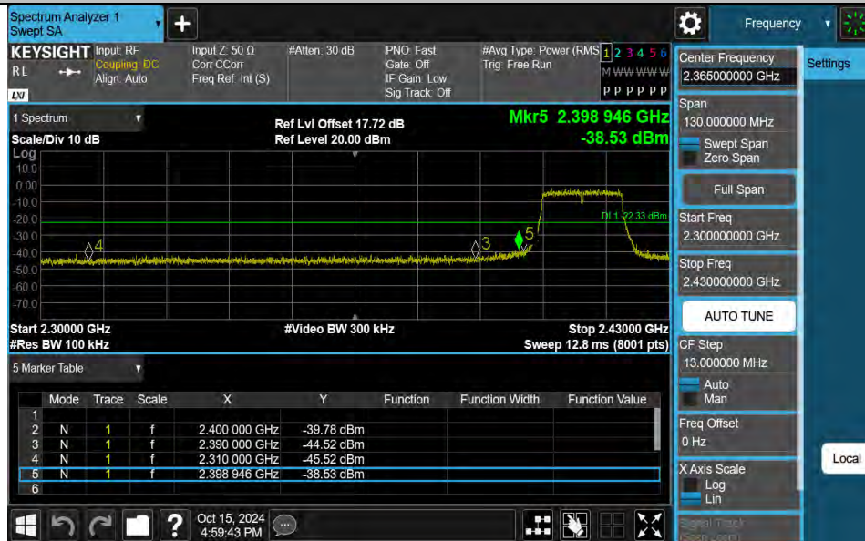
11G-Ant1-2412-PASS
