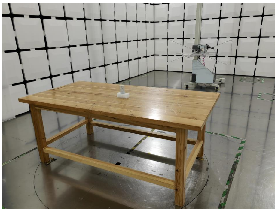
Test Setup For Radiated Emission (30MHz to 1GHz)
