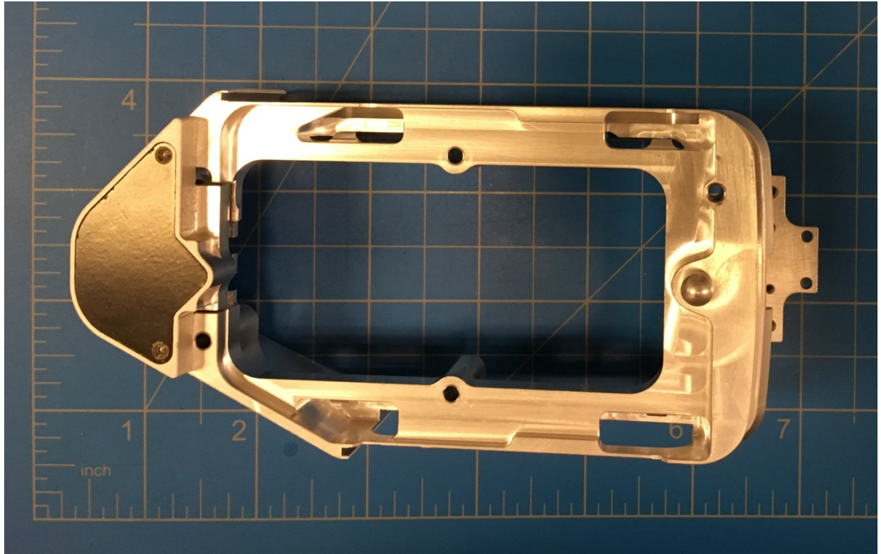
Main Block Bottom
