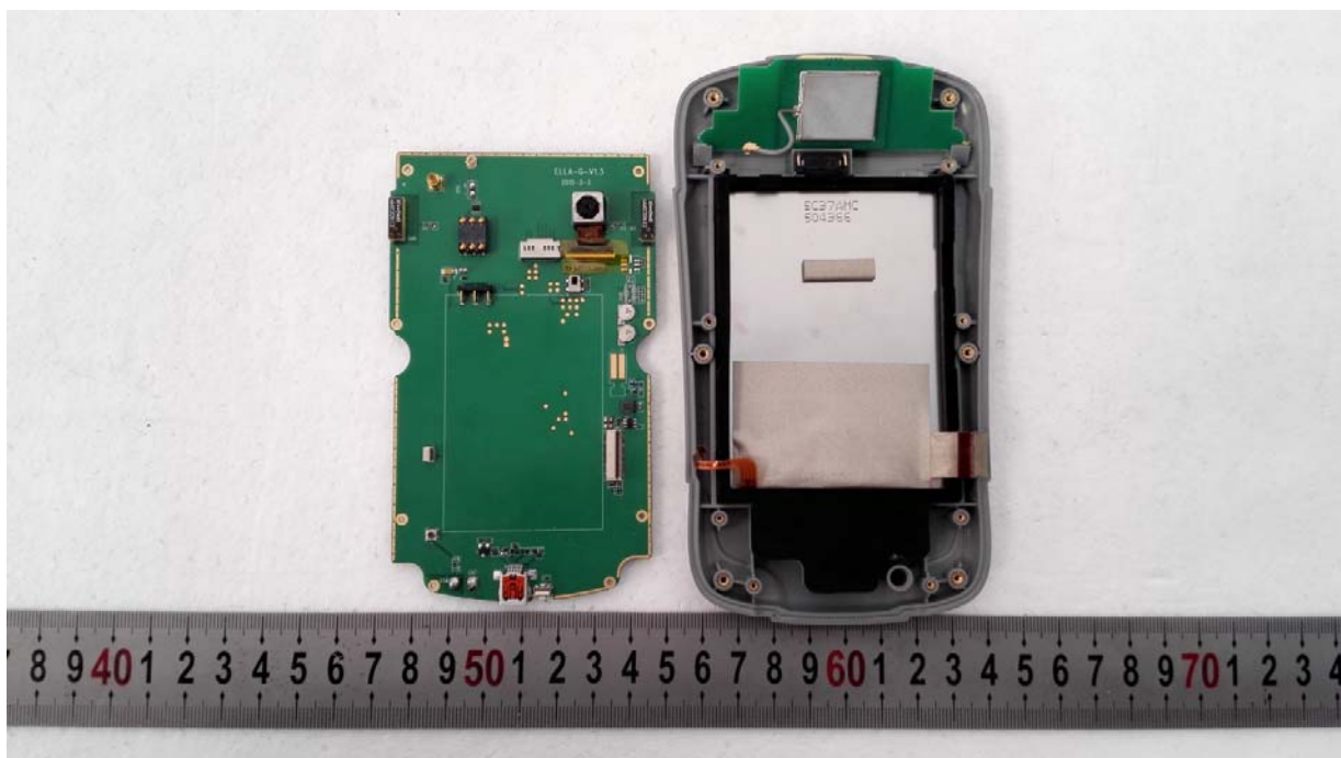
EUT – Cover off View 2
