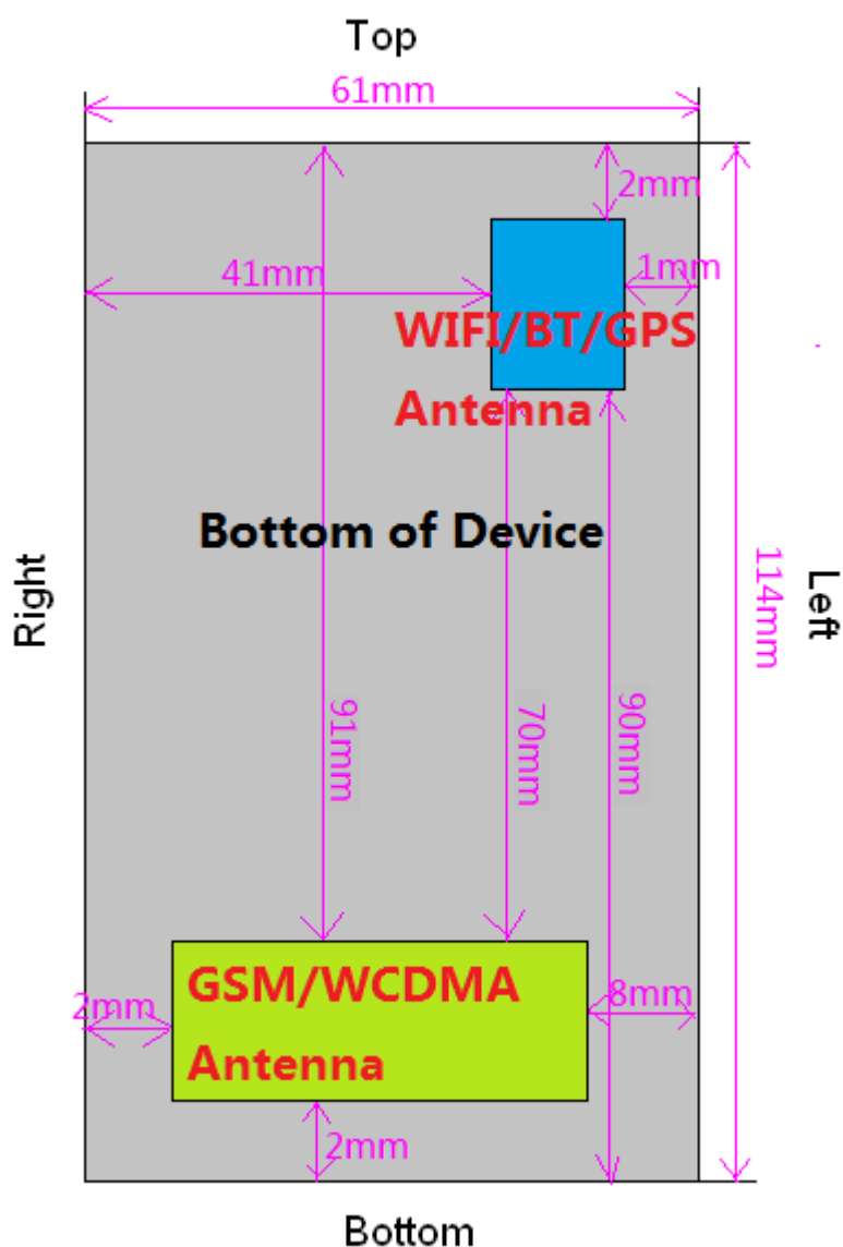
Mobile Test Positions for SAR Testing
