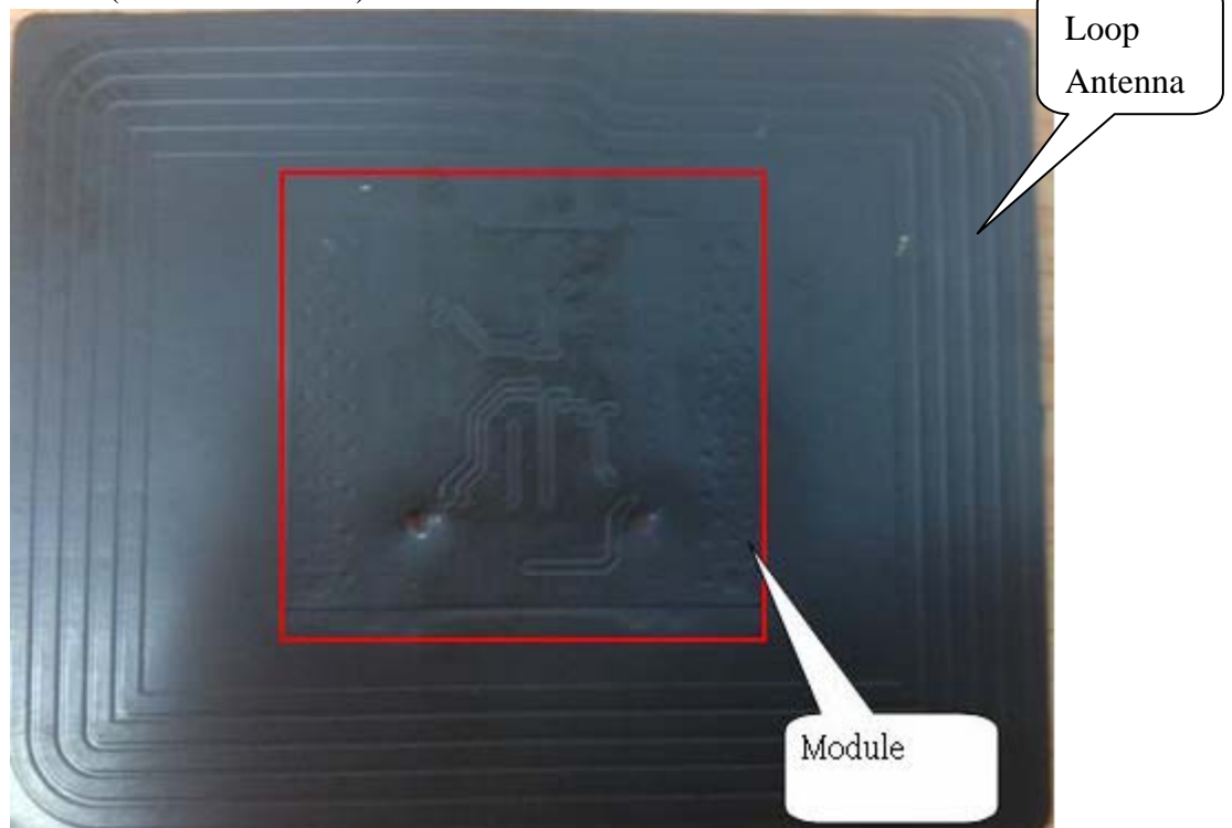
(7) EUT Photo (Back of PC Board)
