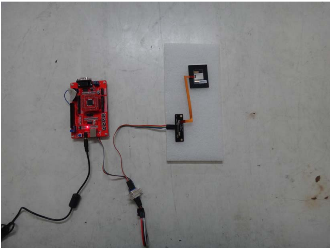
EUT & Test Fixture (8pin cable)
