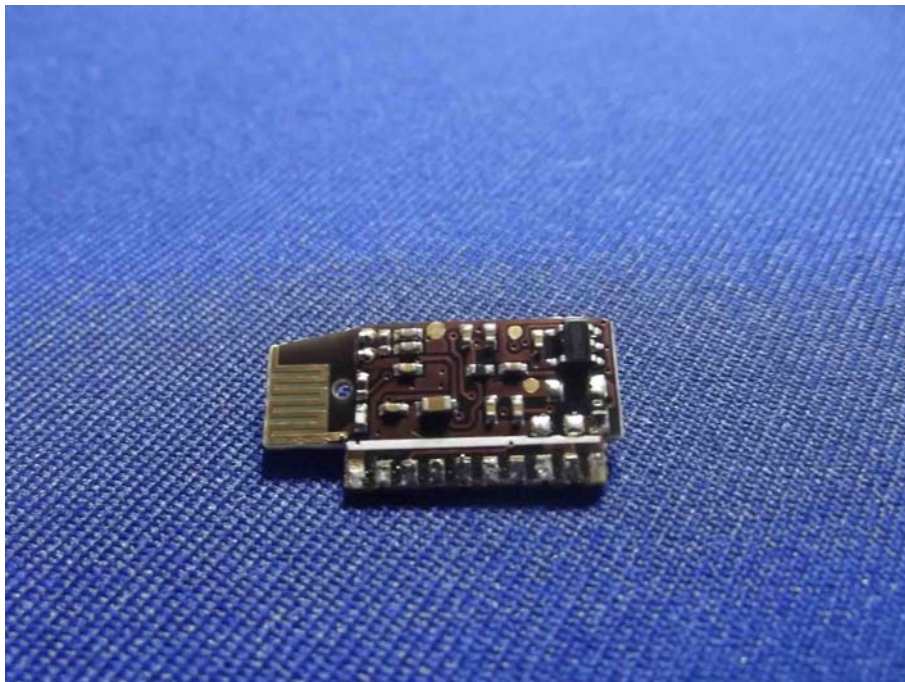
PCB of the EUT-Front View( BT module)
