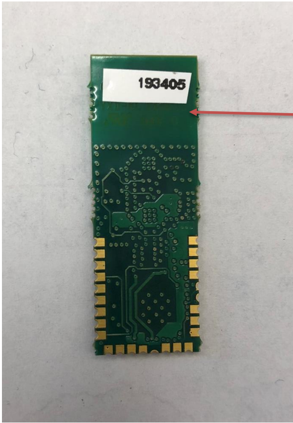
PCB Bottom side of label
