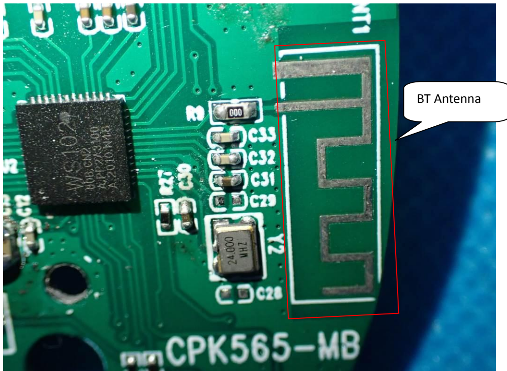
INTERNAL VIEW-16 OF EUT
