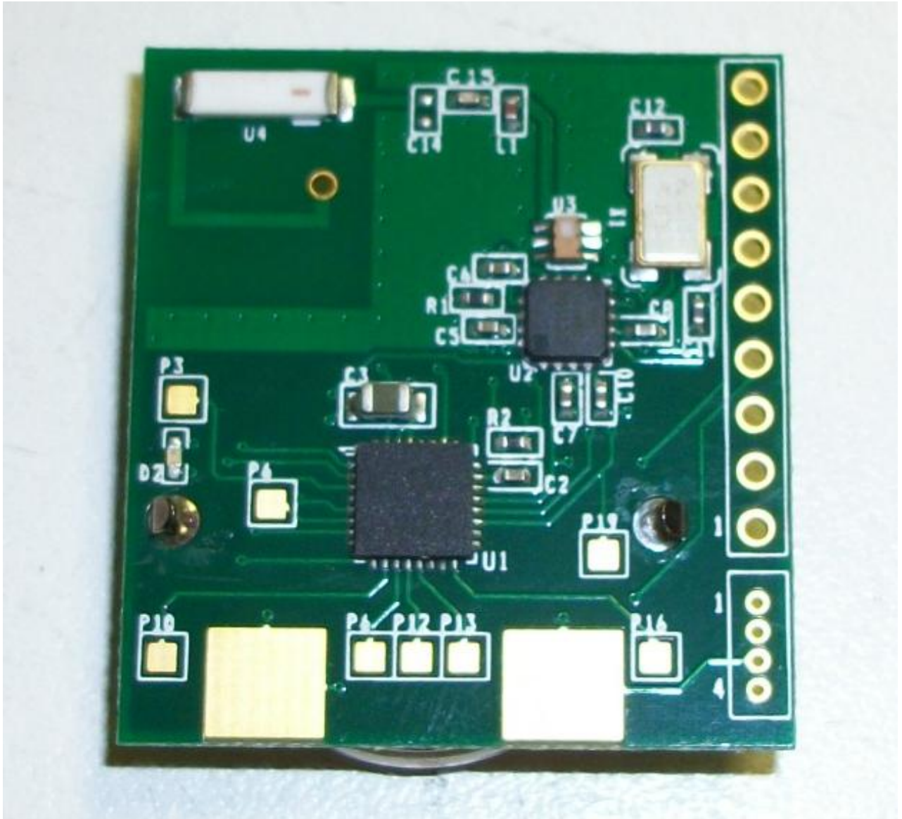
6.4 PCB Component Side View
