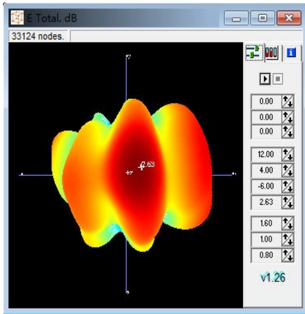
2440MHZ GAIN drawing:
