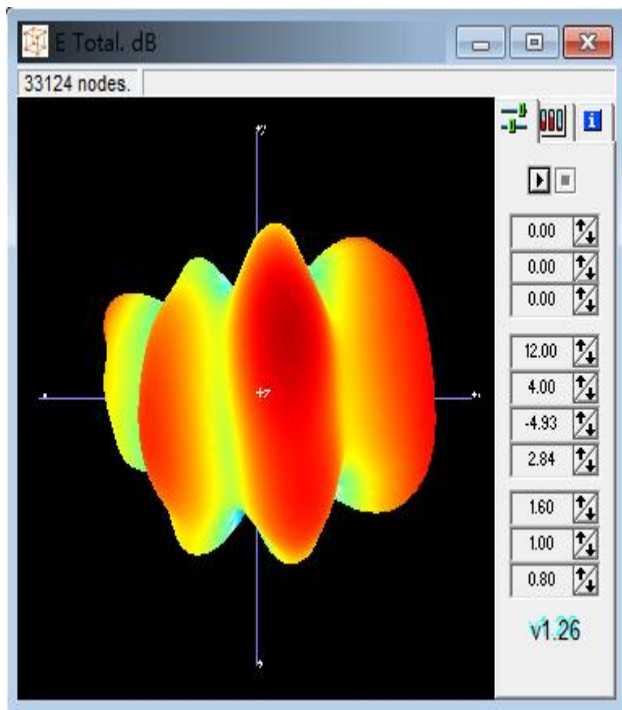
2480MHZ GAIN drawing:
