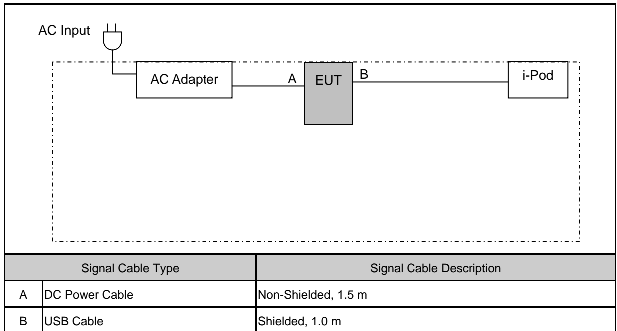
Conducted Emission
