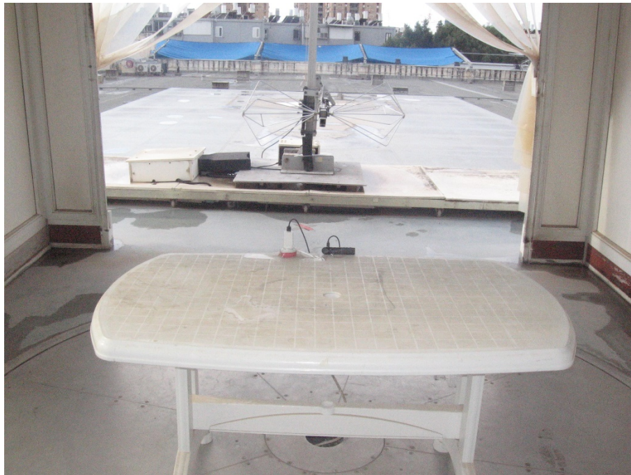
Figure 2. Radiated Emission Test, 30-200MHz
