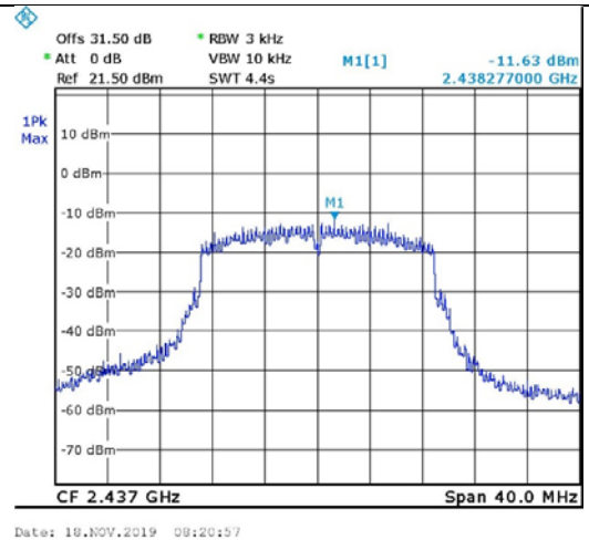
Figure 72. 2437.0 MHz, Wi-fi/n(6.5Mbit/s)
