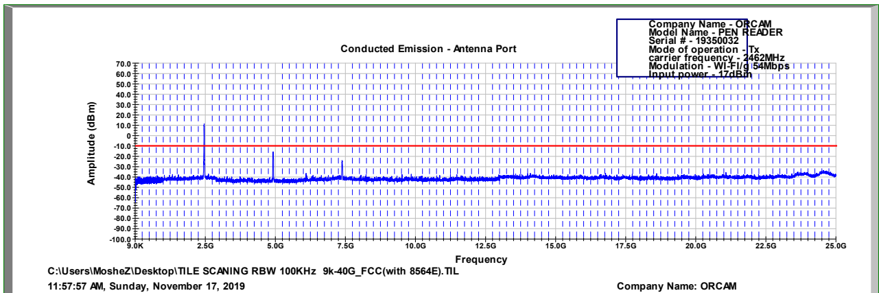
Figure 104 2462.0 MHz, WI-FI/g(54Mbit/s)
