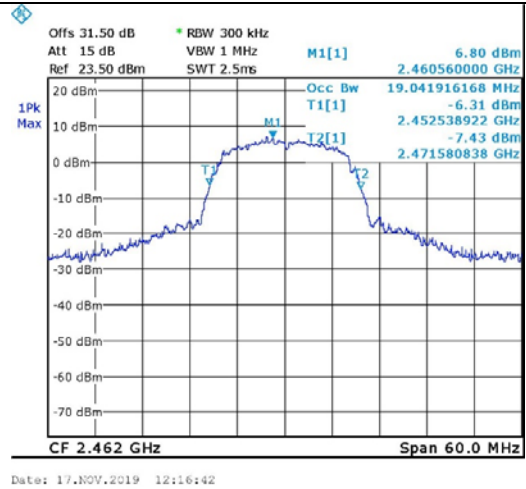
Figure 85. 2462.0 MHz, Wi-fi/g(6Mbit/s)
