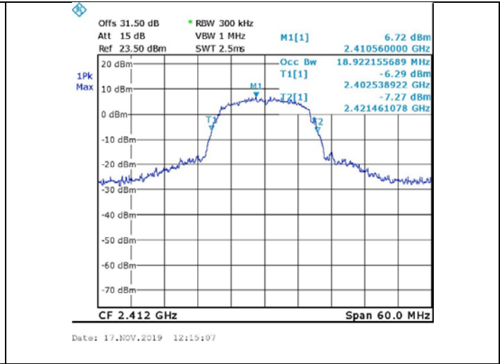
Figure 81. 2412.0 MHz, Wi-fi/g(6Mbit/s)
