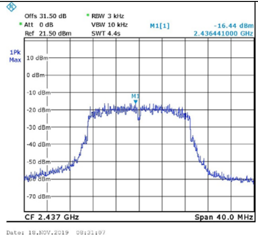
Figure 76. 2437.0 MHz, Wi-fi/n(65Mbit/s)
