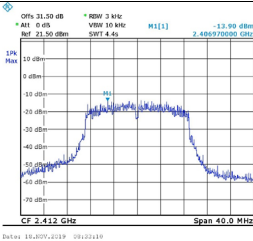
Figure 75. 2412.0 MHz, Wi-fi/n(65Mbit/s)
