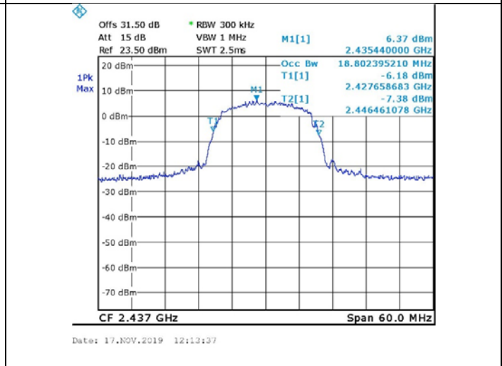
Figure 83. 2437.0 MHz, Wi-fi/g(6Mbit/s)
