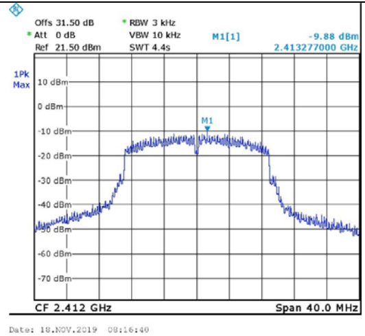
Figure 70. 2412.0 MHz, Wi-fi/n(6.5Mbit/s)
