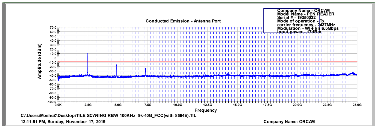
Figure 106 2437.0 MHz, WI-FI/n(6.5Mbit/s)
