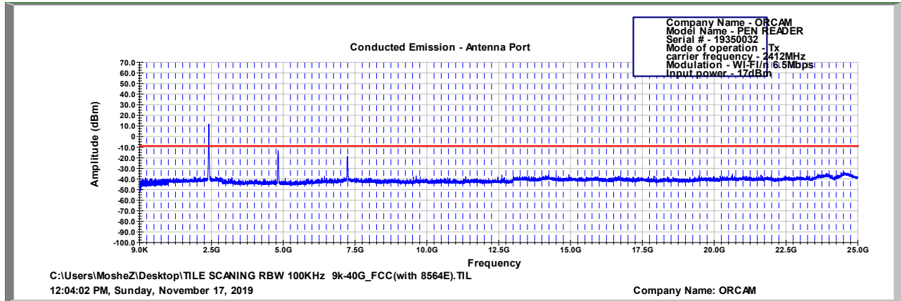
Figure 105 2412.0 MHz, WI-FI/n(6.5Mbit/s)
