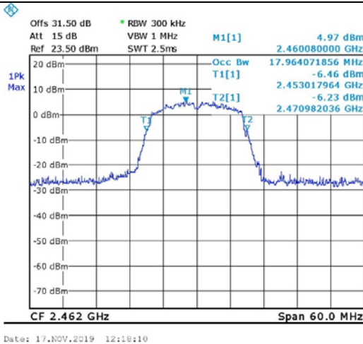
Figure 90. 2462.0 MHz, Wi-fi/g(54Mbit/s)
