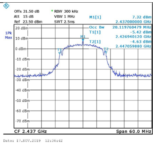
Figure 89. 2437.0 MHz, Wi-fi/n(6.5Mbit/s)
