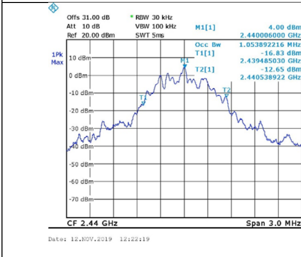
Figure 82. 2440.0 MHz, BLE
