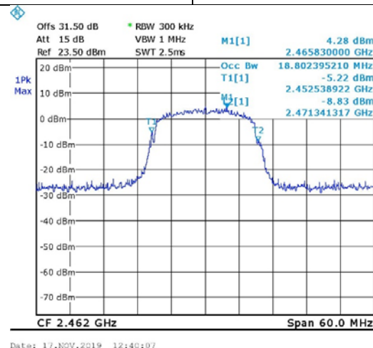
Figure 94. 2462.0 MHz, Wi-fi/n(65Mbit/s)
