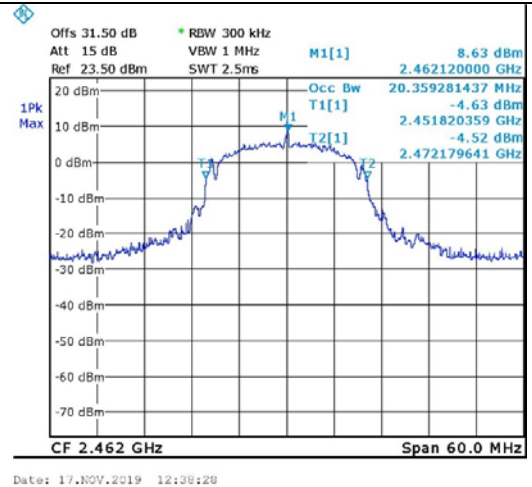
Figure 91. 2462.0 MHz, Wi-fi/n(6.5Mbit/s)
