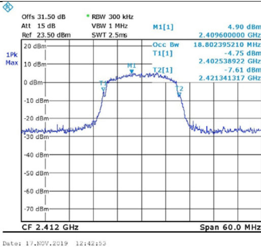
Figure 92. 2412.0 MHz, Wi-fi/n(65Mbit/s)
