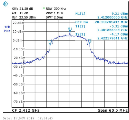
Figure 87. 2412.0 MHz, Wi-fi/n(6.5Mbit/s)
