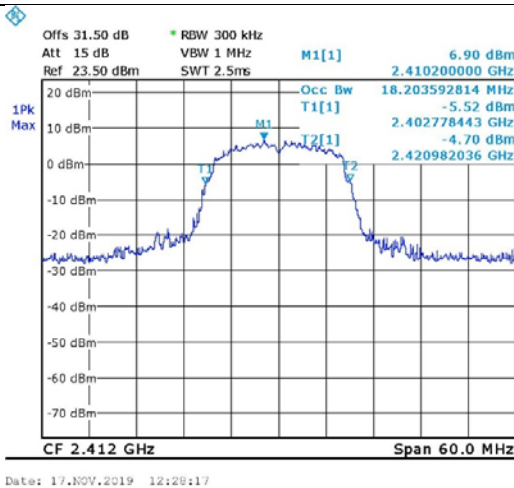
Figure 86. 2412.0 MHz, Wi-fi/g(54Mbit/s)
