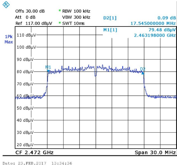
Figure 28 — 2472.0MHz - Wi-Fi/n
