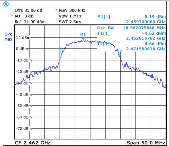
Figure 85. 2462.0 MHz, Wi-fi/g(6Mbit/s)
