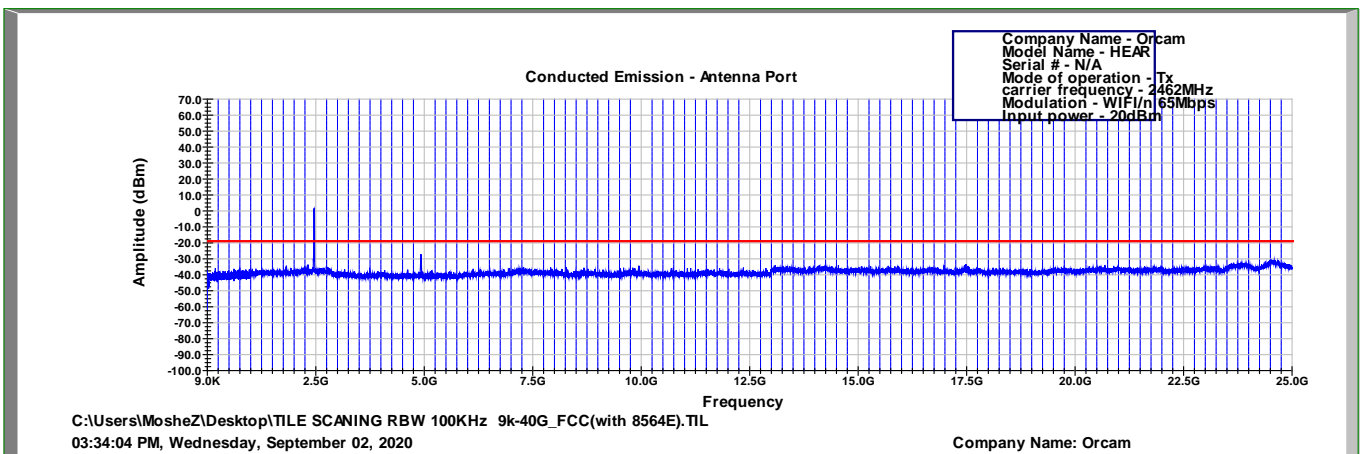
Figure 110 2462.0 MHz, WI-FI/n(65Mbit/s)
