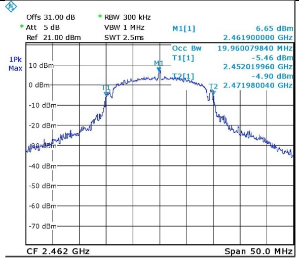
Figure 91. 2462.0 MHz, Wi-fi/n(6.5Mbit/s)
