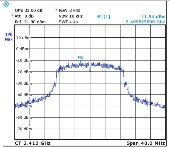
Figure 70. 2412.0 MHz, Wi-fi/n(6.5Mbit/s)
