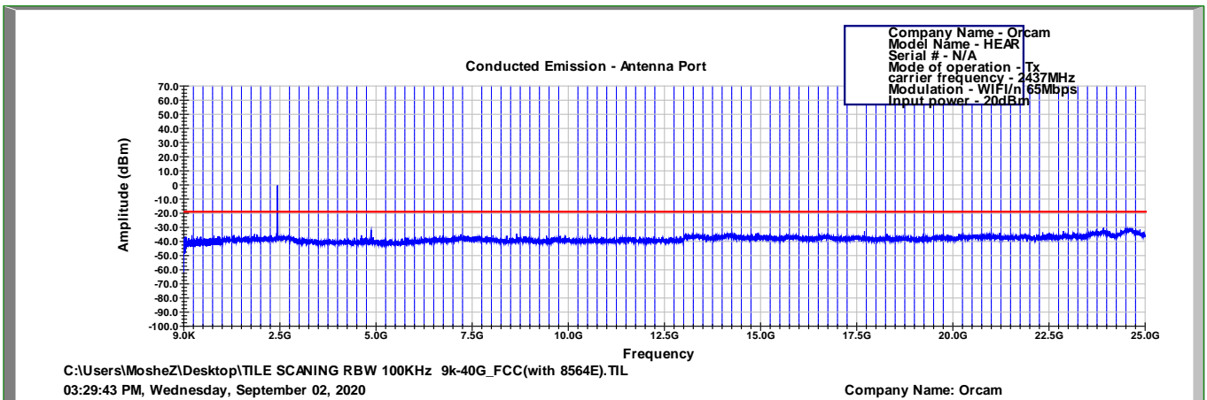
Figure 109 2437.0 MHz, WI-FI/n(65Mbit/s)
