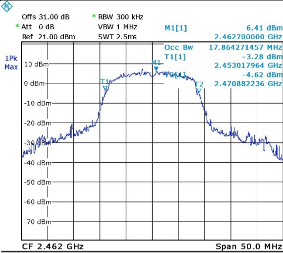
Figure 90. 2462.0 MHz, Wi-fi/g(54Mbit/s)
