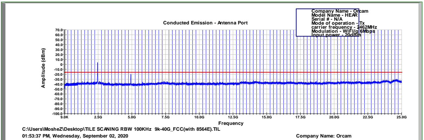
Figure 101 2462.0 MHz, WI-FI/g(6Mbit/s)
