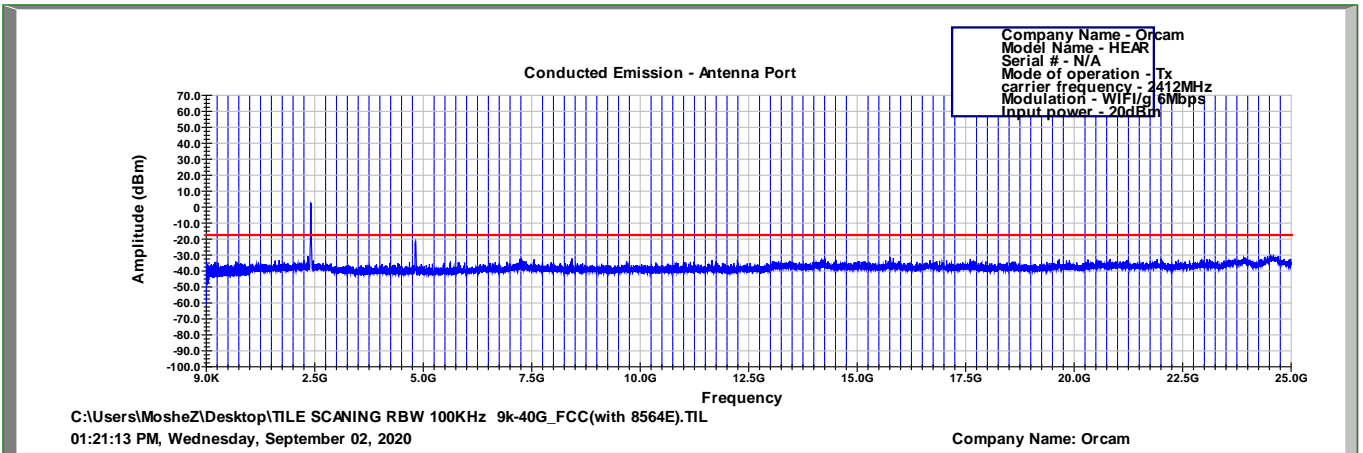
Figure 99 2412.0 MHz, WI-FI/g(6Mbit/s)
