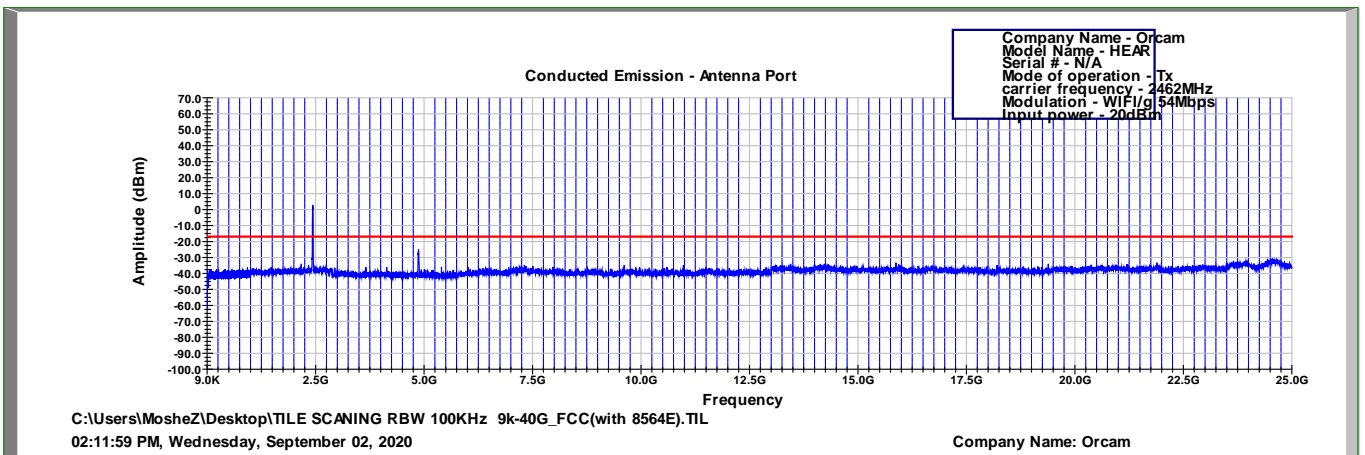
Figure 104 2462.0 MHz, WI-FI/g(54Mbit/s)
