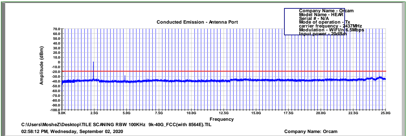
Figure 106 2437.0 MHz, WI-FI/n(6.5Mbit/s)
