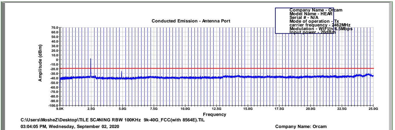
Figure 107 2462.0 MHz, WI-FI/n(6.5Mbit/s)
