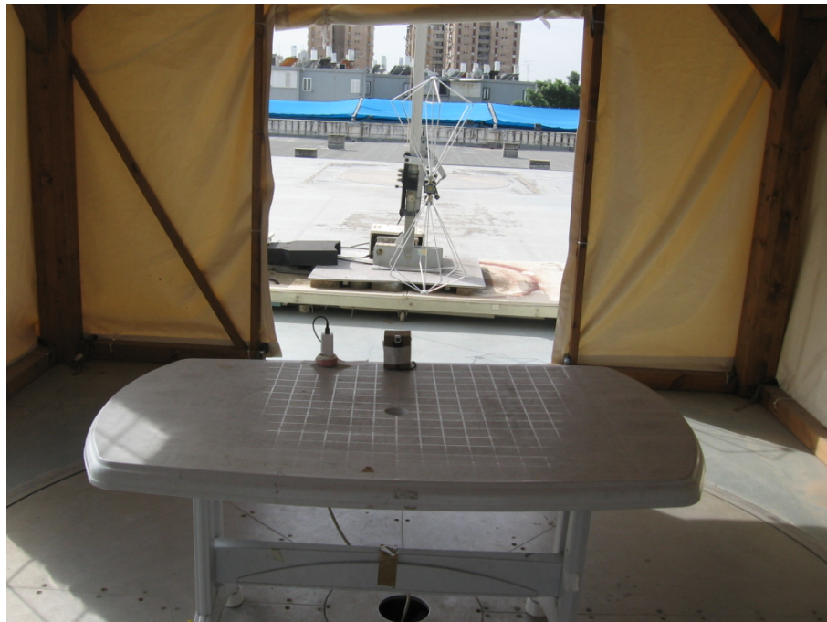
Figure 7. Radiated Emission Test, 30-200MHz
