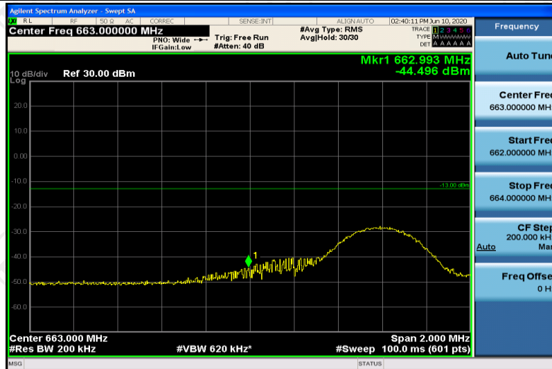
Band71-10MHz-16QAM-133172-1RB#0
