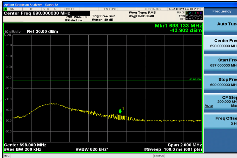
Band71-10MHz-16QAM-133422-1RB#49
