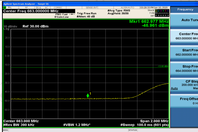
Band71-20MHz-16QAM-133222-1RB#0
