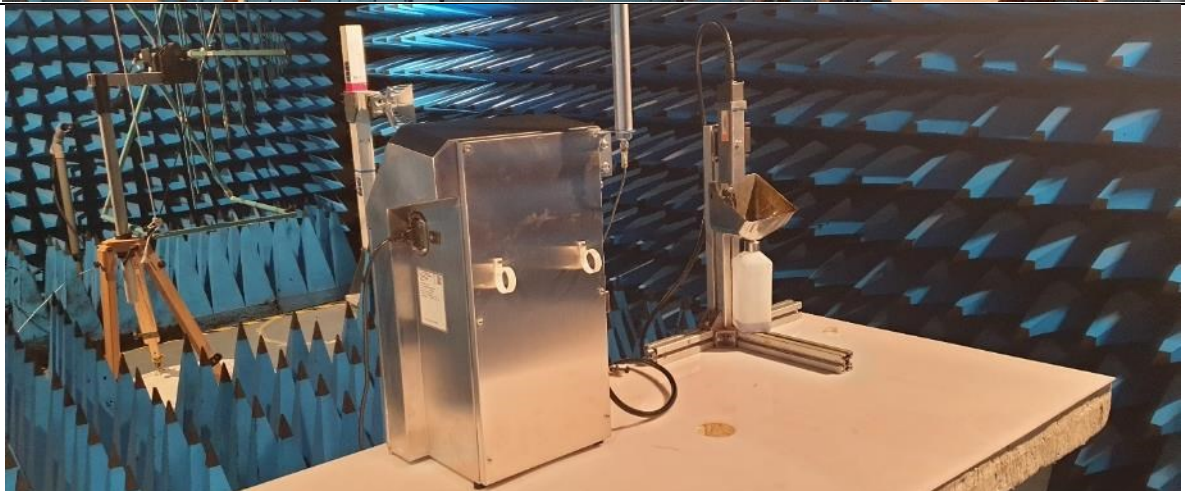
Test setup in anechoic chamber – Frequency <1GHz
