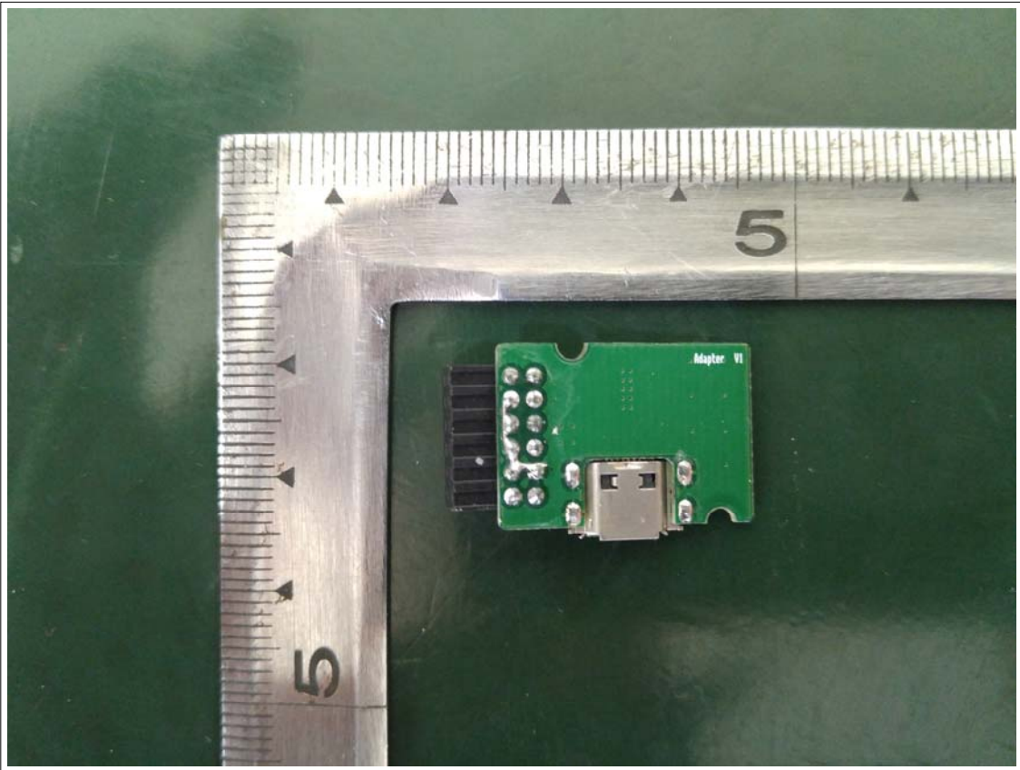
View of Side PCB(Bottom)
