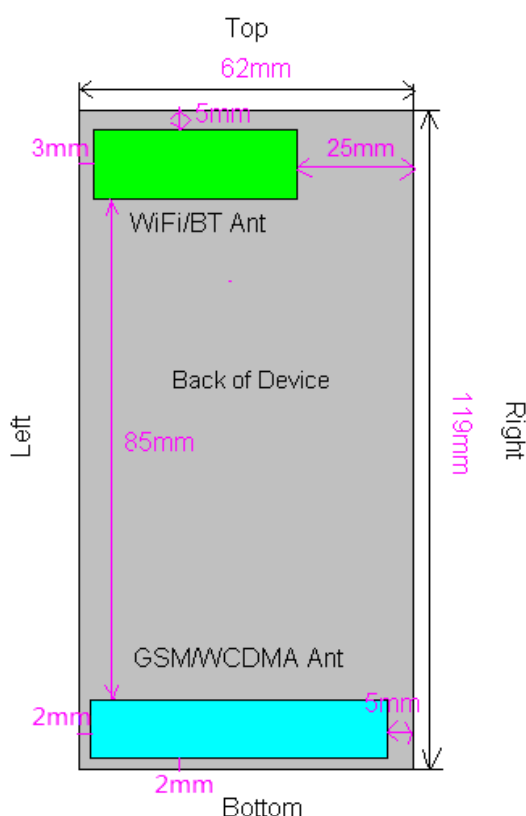
Mobile Hotspot Sides for SAR Testing
