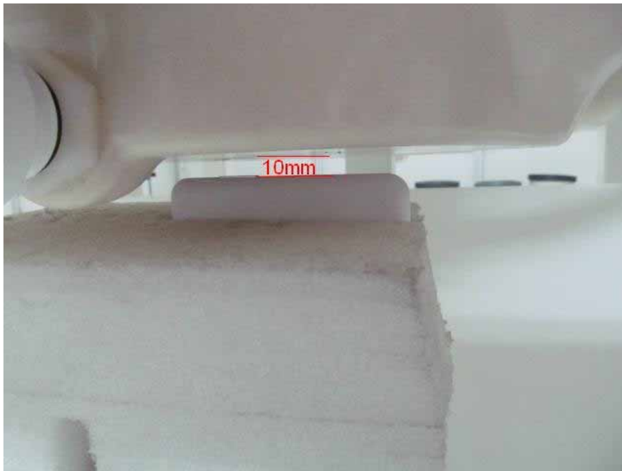
Body SAR Left Side 10mm for WIFI
