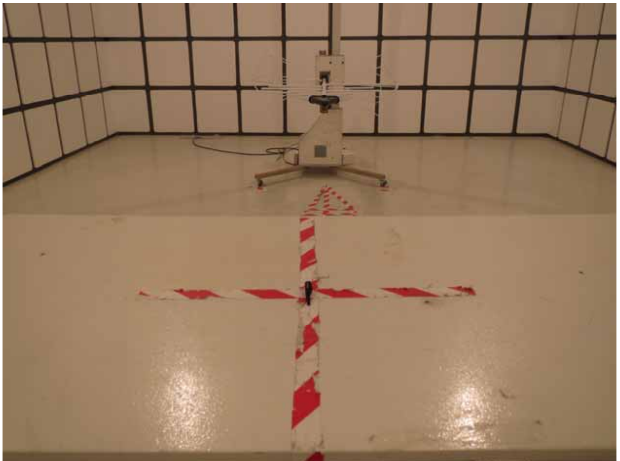
Radiated emissions test(transmitting)
