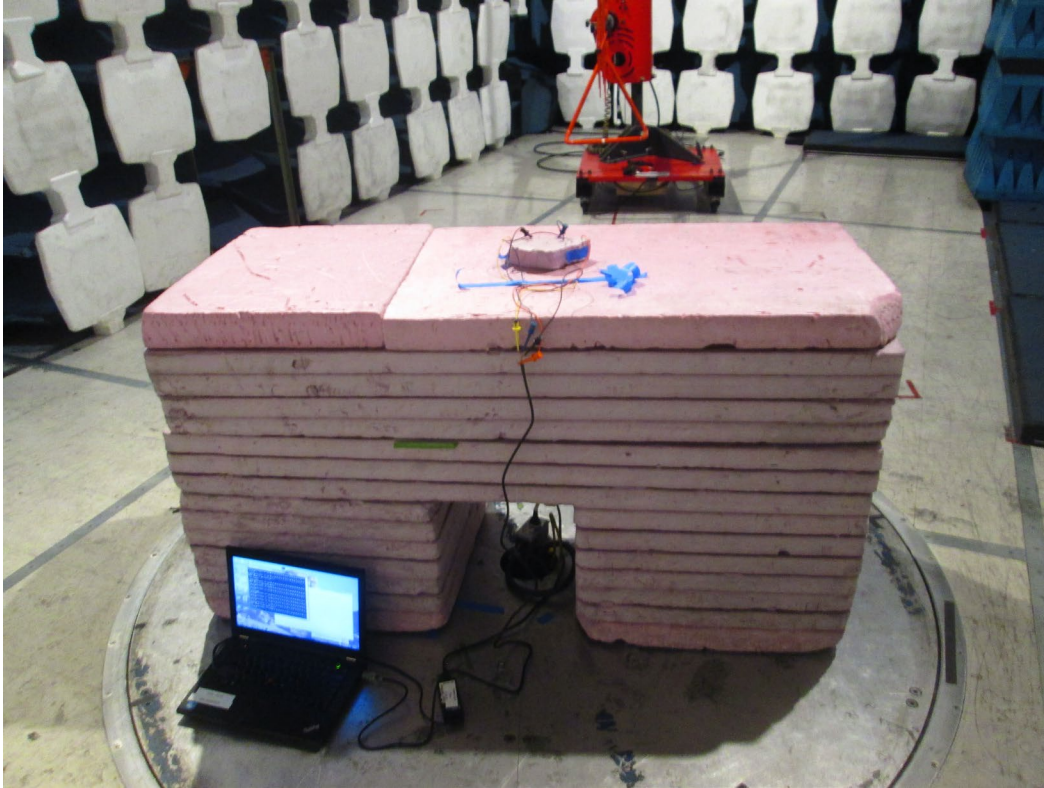
Y-Plane RSE 30MHz – 1GHz Front
