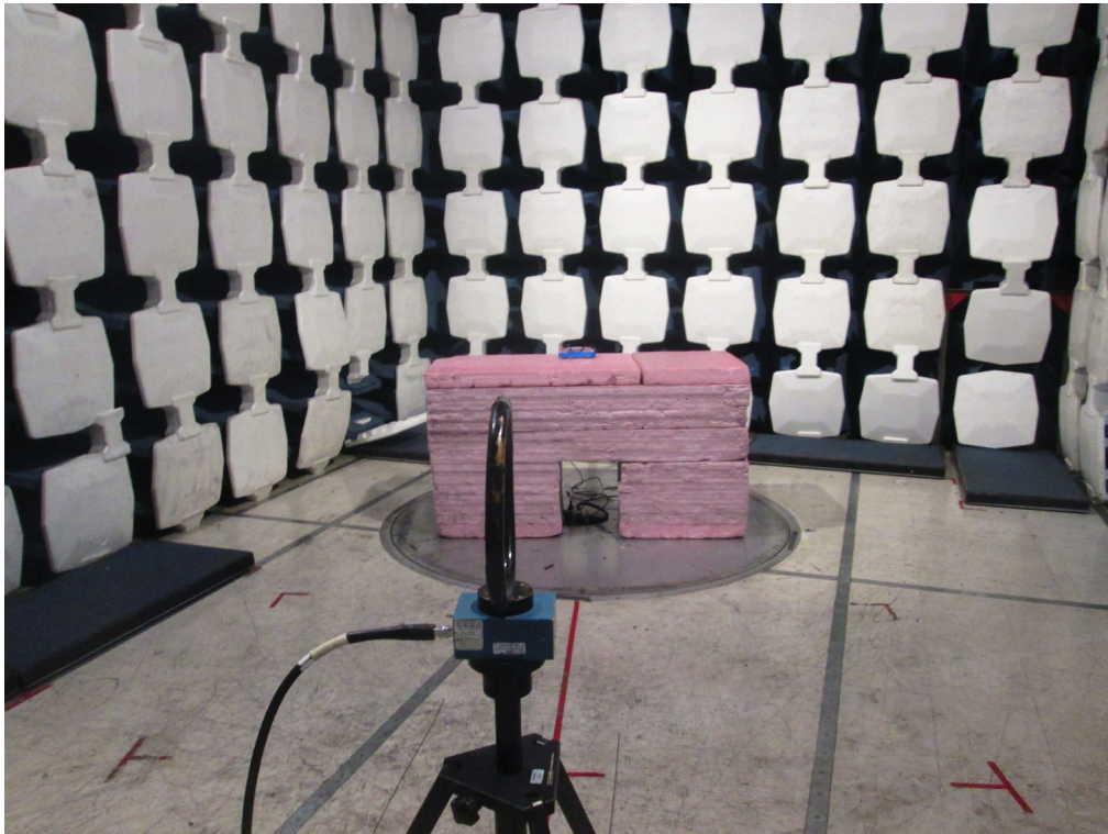
Y-Plane RSE Below 30MHz Front
