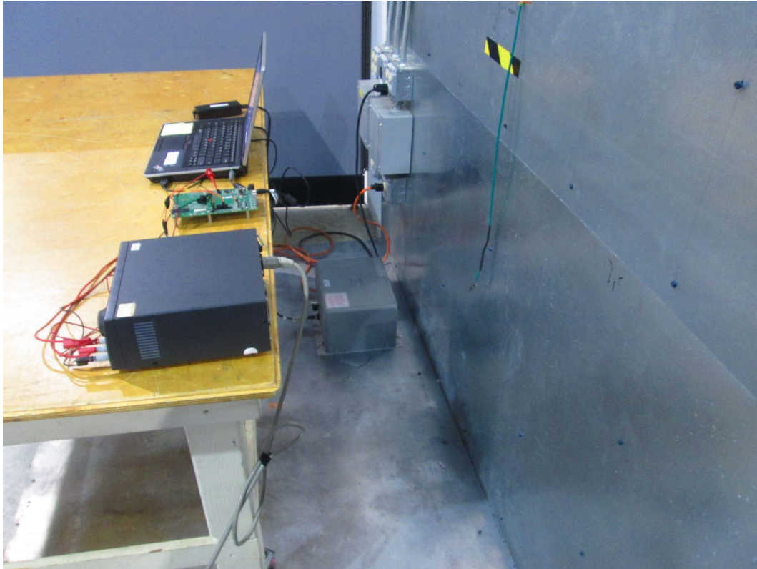
AC Mains Conducted Emissions Front
