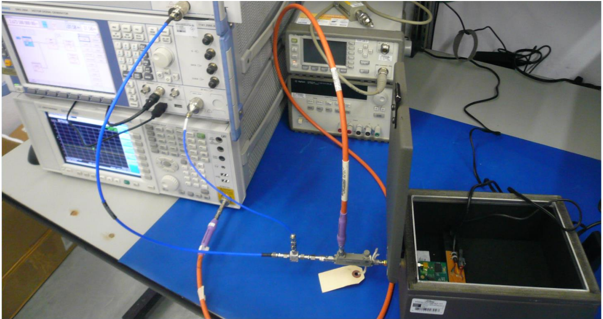
Figure 7: RF Bench Test Setup
