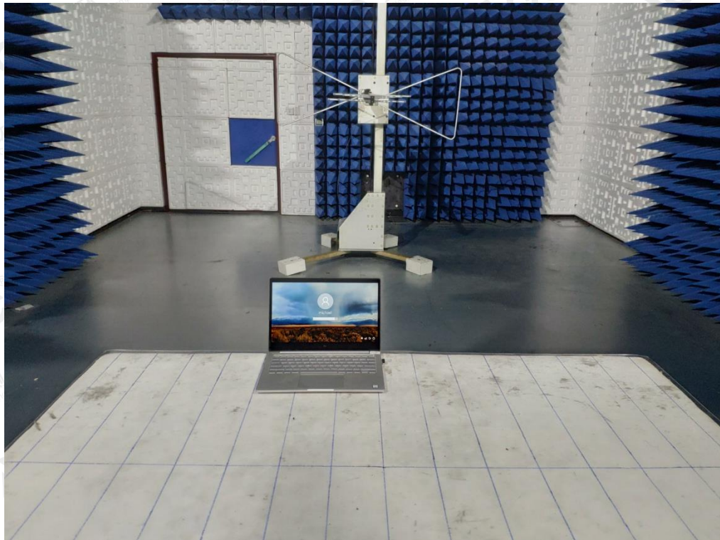
FCC RADIATED EMISSION TEST SETUP BELOW 1GHZ
